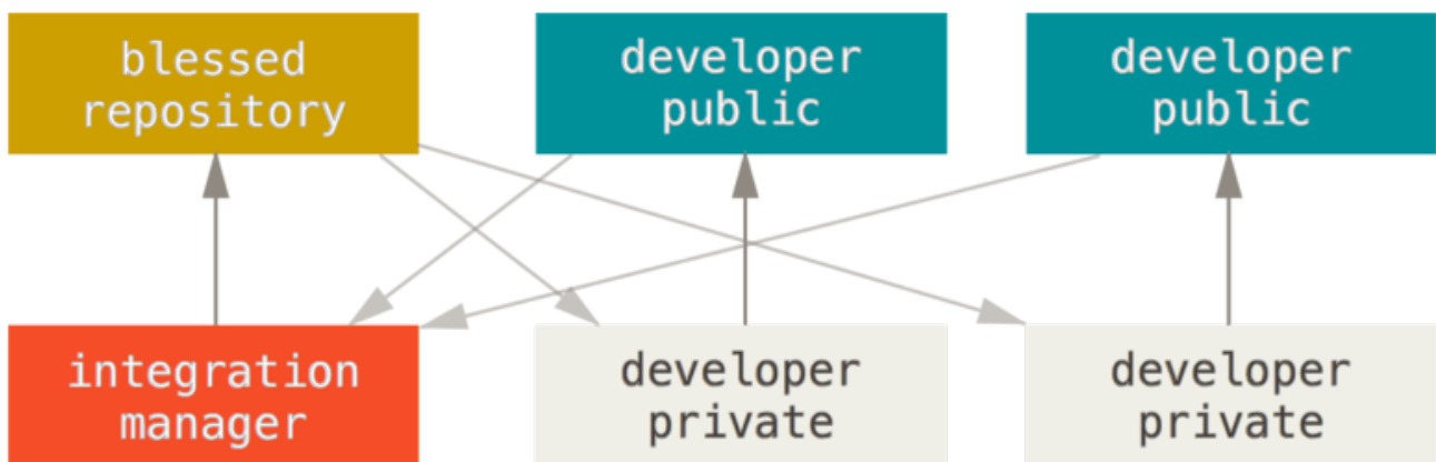
Figura 55. Integration-manager workflow.
