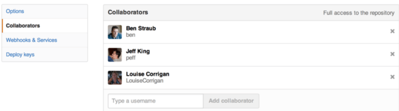
Figura 114. Repository collaborators.
