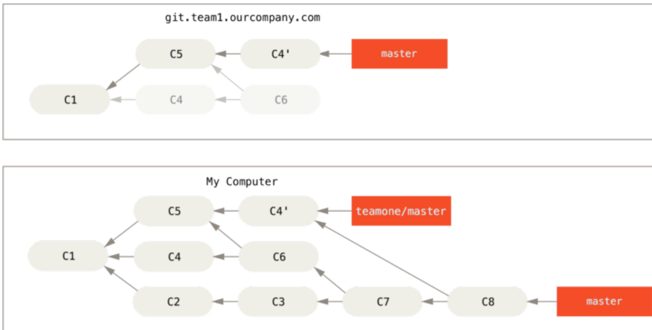
Figura 47. You merge in the same work again into a new merge commit
