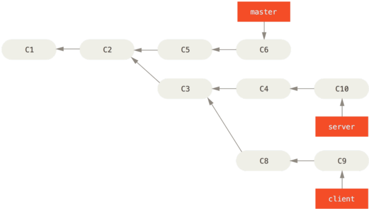
Figura 39. A history with a topic branch off another topic branch
