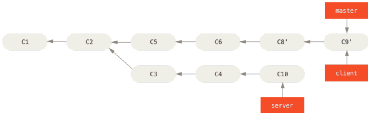
Figura 41. Fast-forwarding your master branch to include the client branch changes
