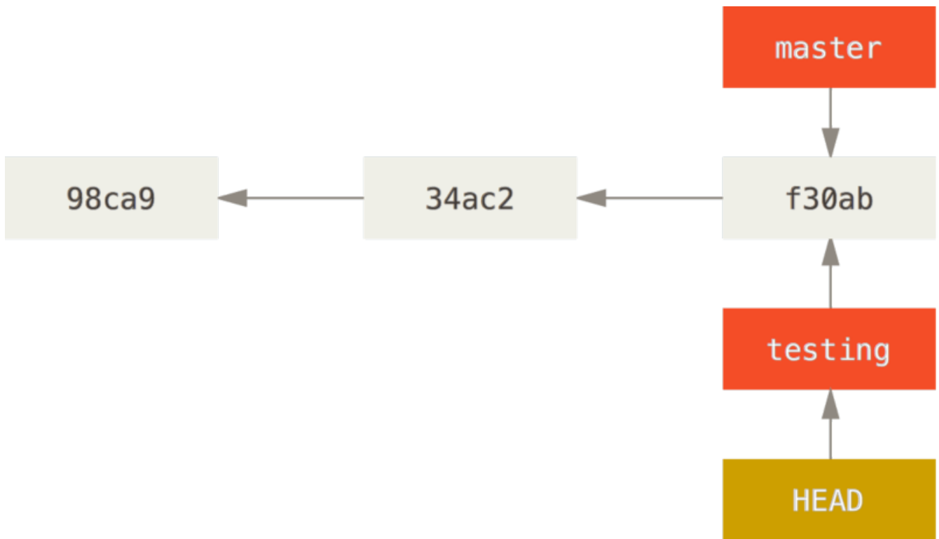
Figura 14. HEAD points to the current branch
