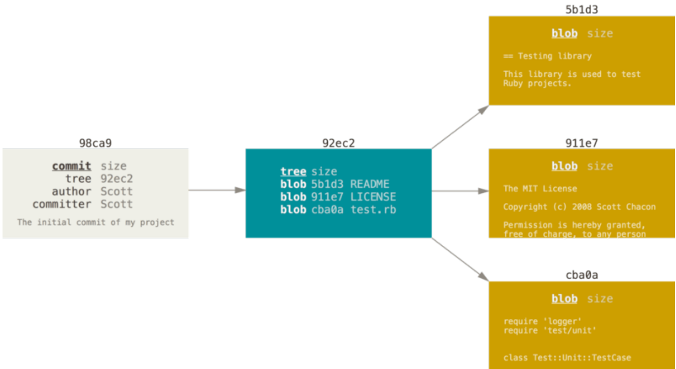
Figura 9. A commit and its tree
