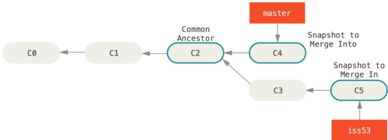
Figura 24. Three snapshots used in a typical merge
