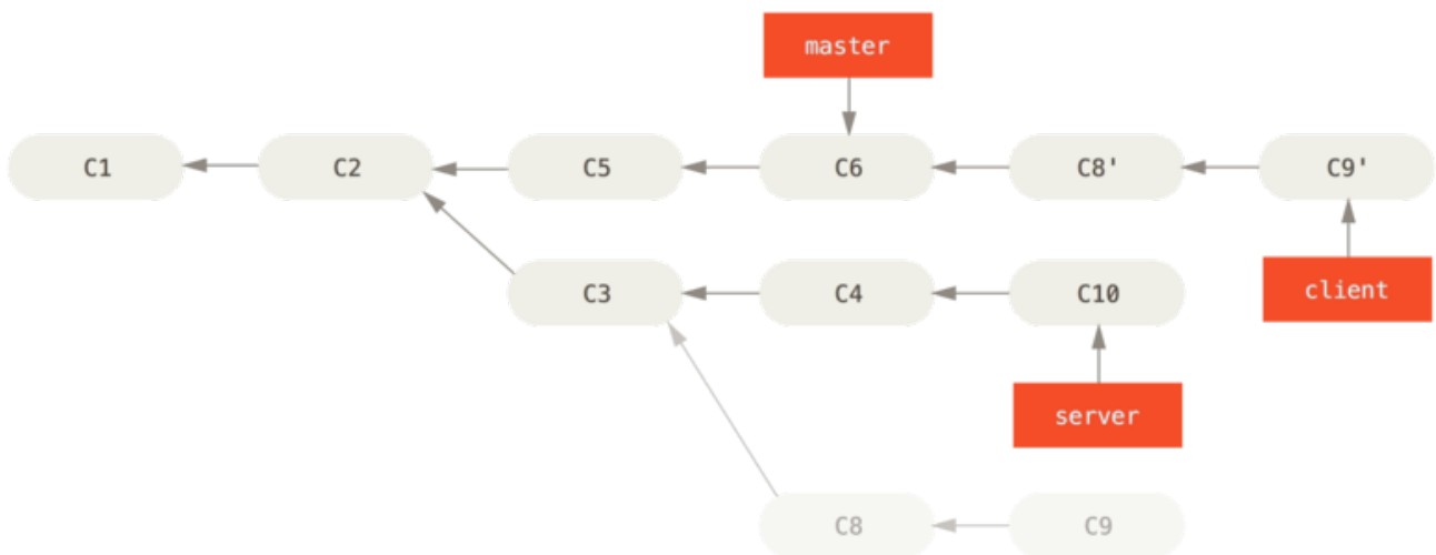
Figura 40. Rebasing a topic branch off another topic branch
