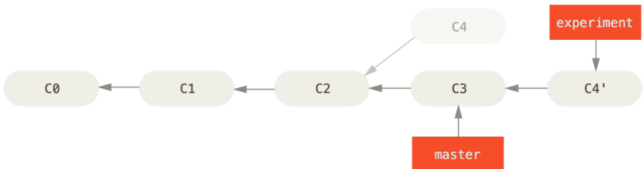
Figura 37. Rebasing the change introduced in C4 onto C3
