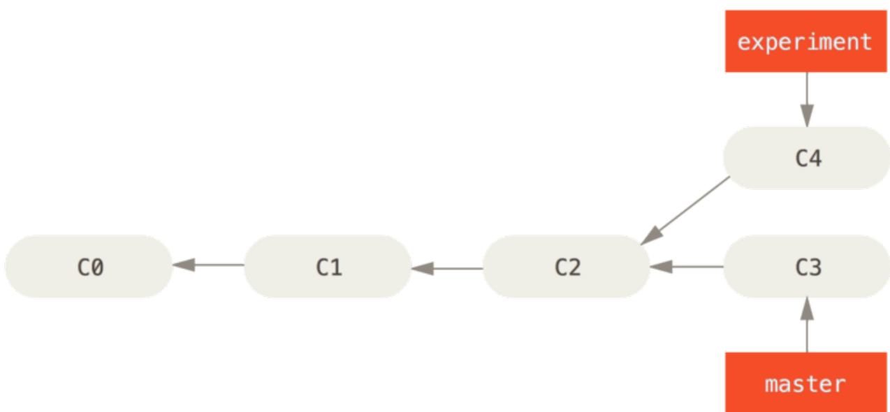
Figura 35. Simple divergent history
