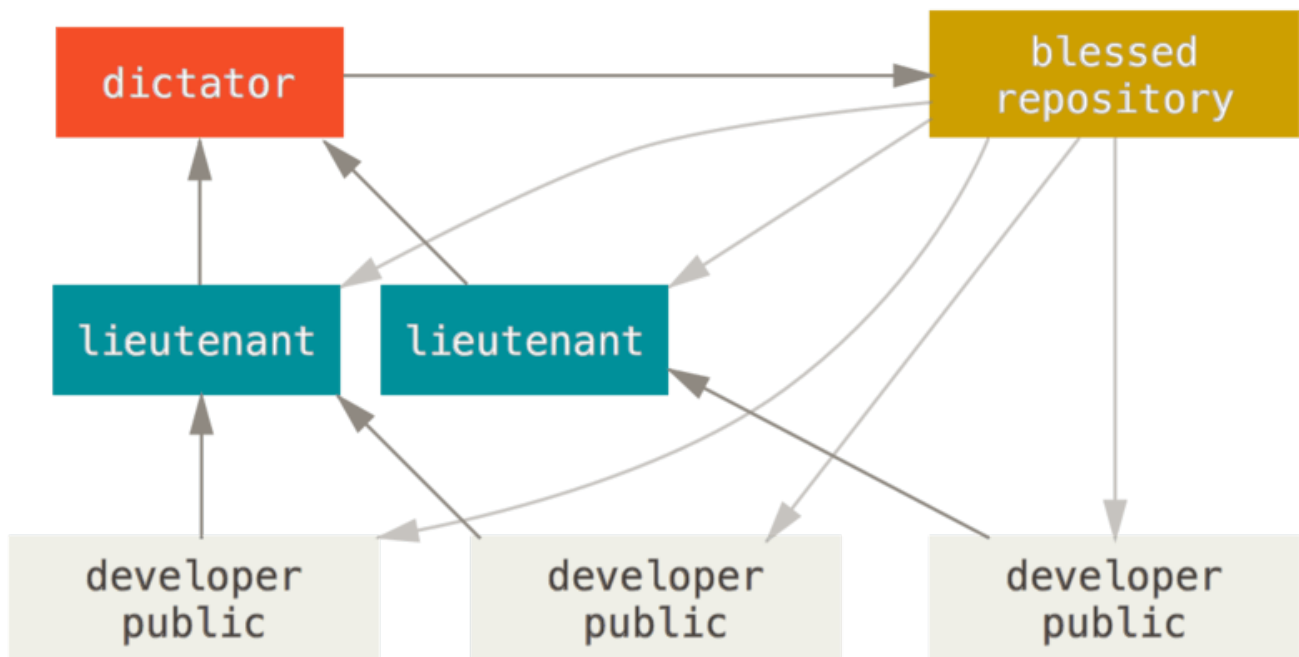
Figura 56. Benevolent dictator workflow.
