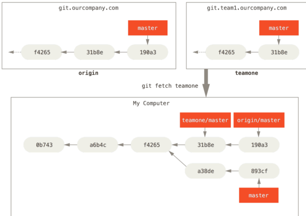
Figura 34. Remote tracking branch for teamone/master
