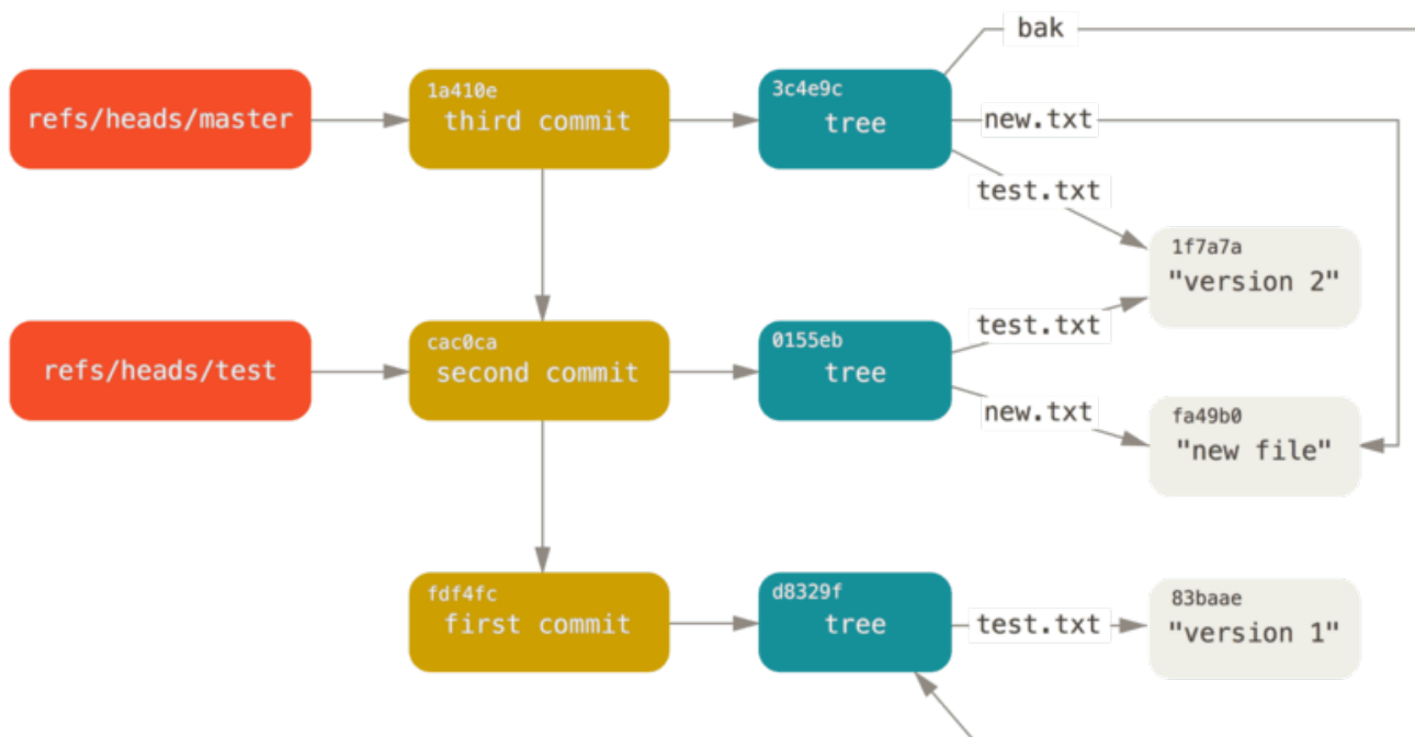
Figura 152. Git directory objects with branch head references included.
