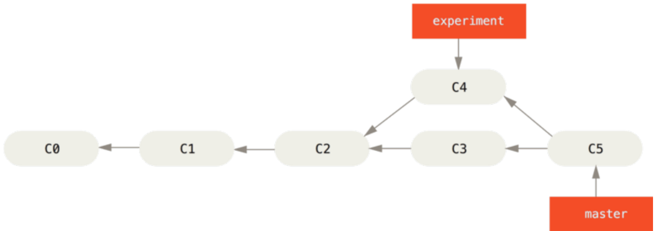
Figura 36. Merging to integrate diverged work history
