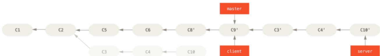
Figura 42. Rebasing your server branch on top of your master branch
