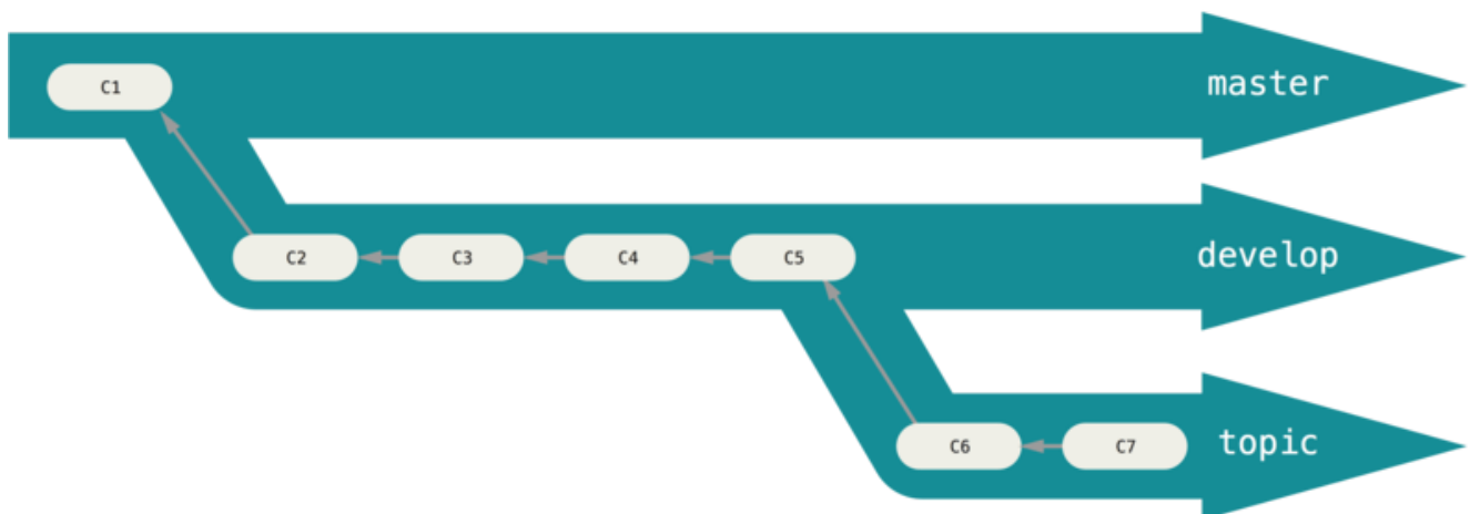
Figura 27. A "silo" view of progressive-stability branching
