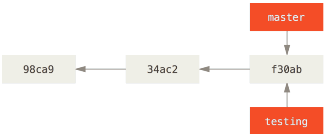
Figura 12. Two branches pointing into the same series of commits
