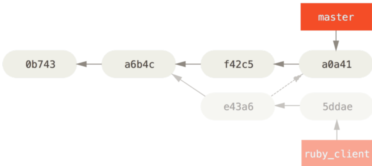
Figura 81. History after cherry-picking a commit on a topic branch.
