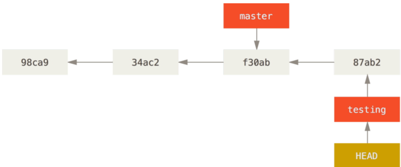
Figura 15. The HEAD branch moves forward when a commit is made
