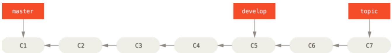
Figura 26. A linear view of progressive-stability branching
