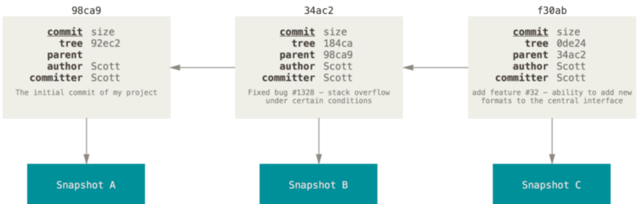
Figura 10. Commits and their parents
