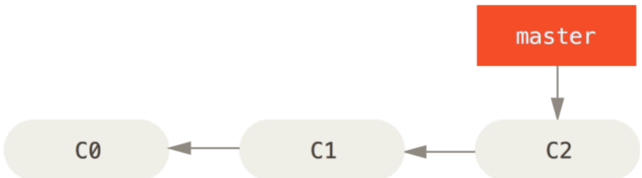
Figura 18. A simple commit history
