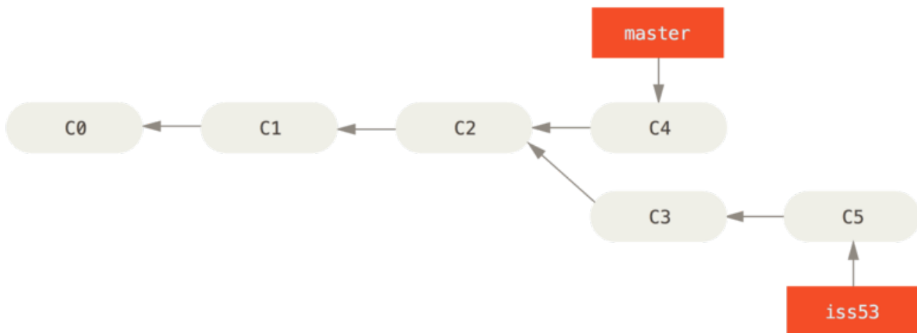
Figura 23. Work continues on iss53
