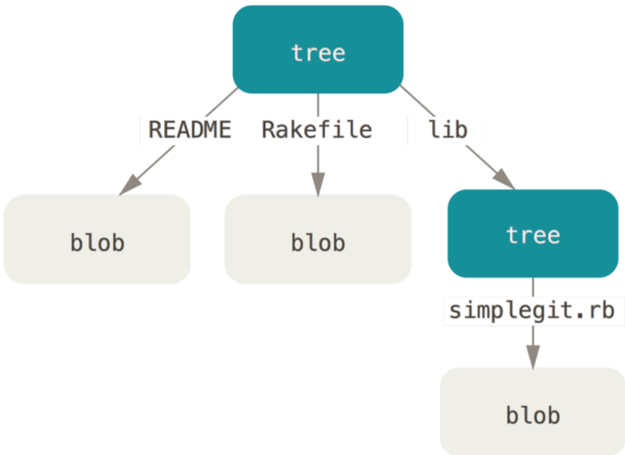
Figura 149. Simple version of the Git data model.
