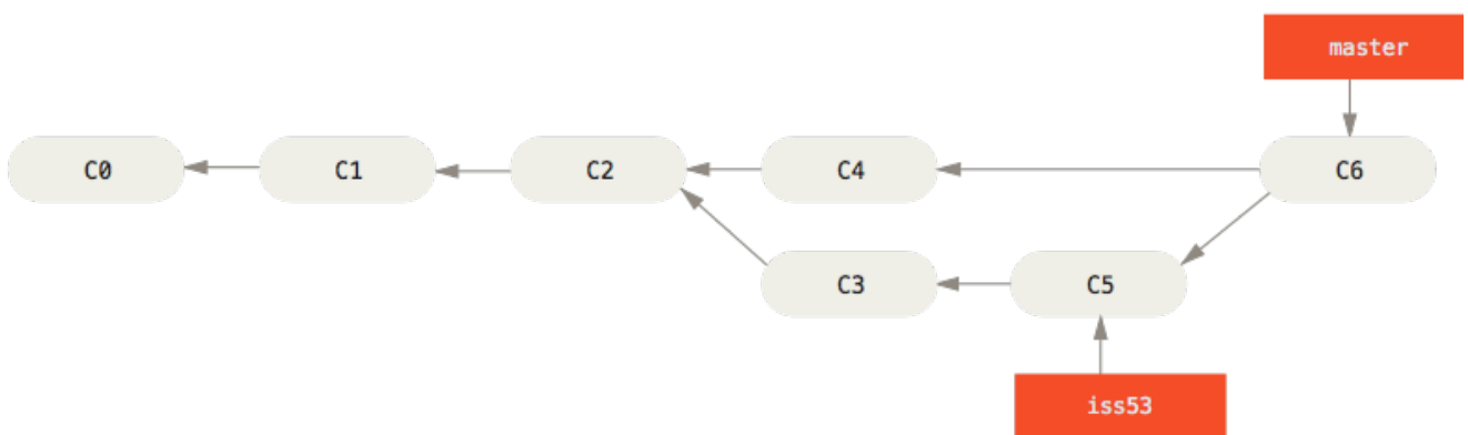
Figura 25. A merge commit
