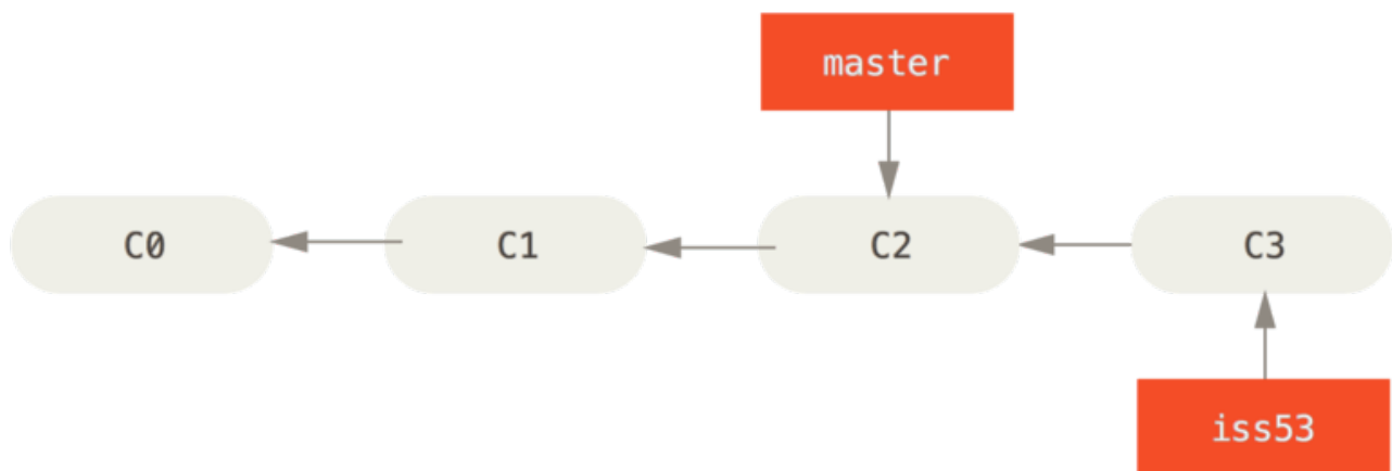
Figura 20. The iss53 branch has moved forward with your work
