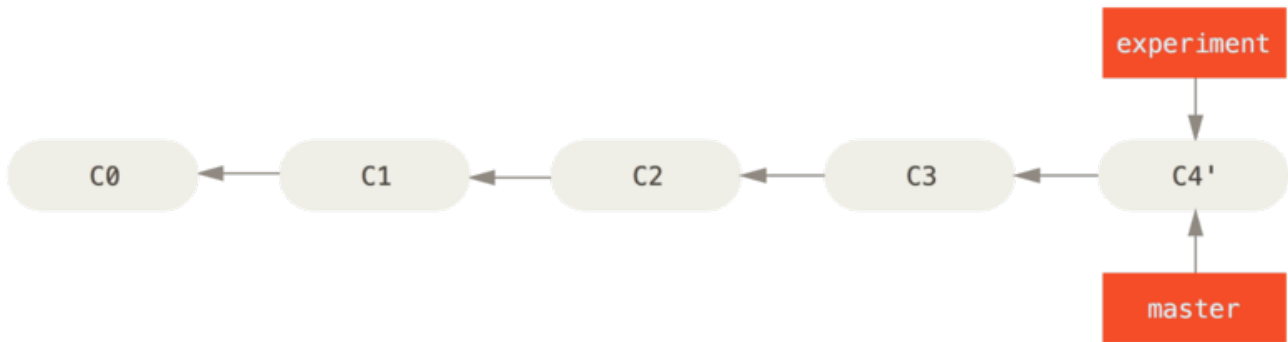
Figura 38. Fast-forwarding the master branch
