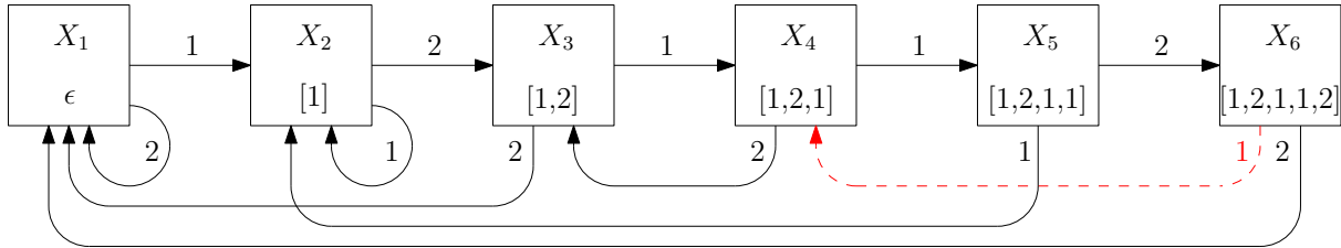
335 Figure 2: Illustration to Example 4.3: the automaton marking occurrences of the pattern 121121.
