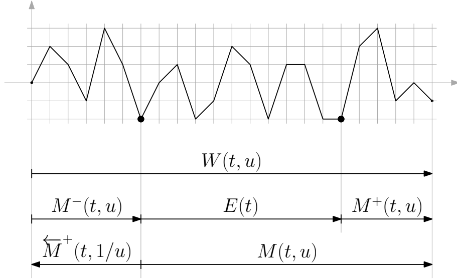
555 Figure 4: The Wiener–Hopf factorization of a walk: W = M^-EM^+ , a product of a reversed- 556 meander, an excursion, and a positive meander. See e.g. [44] for the importance of this 557 factorization for lattice path enumeration. This has further consequences on pattern avoidance 558 when one reverses the time.
