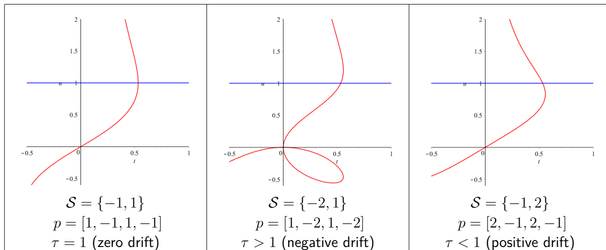
800 Figure 5: For the asymptotics of meanders, the key is to compare the location of the singularity \rho 801 (the branching point of u_1, v_1 ) with the zeroes of K(t, 1) , and the values t such that u_i(t) = 1 .
