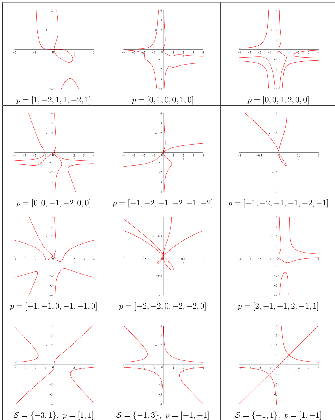
430 Table 2: Several examples that demonstrate the diversity of the behaviour of real branches of 431 K(t, u) = 0 . In all the examples the set of steps is \mathcal{S} = \{-2, -1, 0, 1, 2\} (except for the last 432 three examples, where \mathcal{S} is indicated explicitly), and the pattern p is as indicated. The kernel 433 K may also have some complex branches (large or small): they are not shown in the figure, but 434 do play a role in our formulas.
