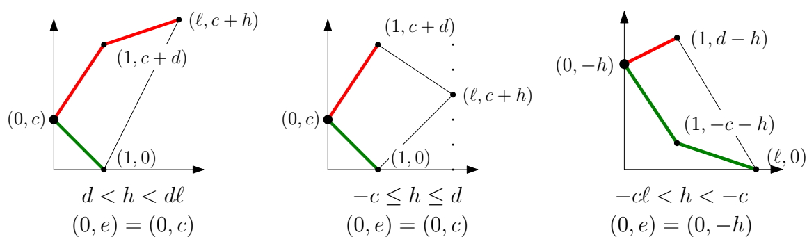
Figure 3: Three possibilities for the Newton polygon of the kernel K(t, u) . This classification depends on the final altitude h of the pattern p , and is exhaustive if R(t, u) = 1 . Each point (i, j) corresponds to a monomial t^i u^j of the numerator of K . The slopes of the convex hull segments on the left give the Puiseux behaviour at 0 of the small and large roots u_i and v_j .
