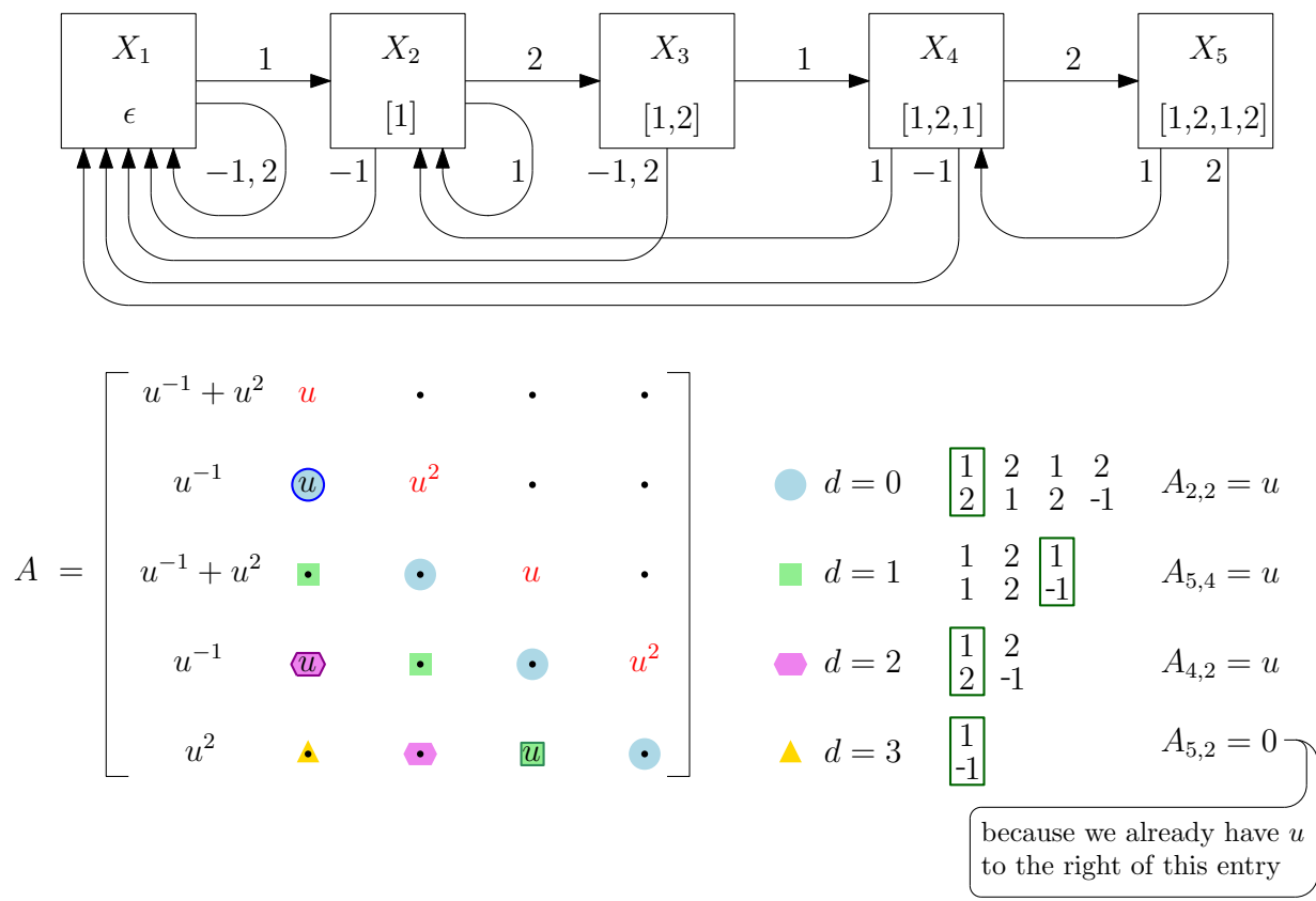
236 Figure 1: The automaton and the adjacency matrix A for \mathcal{S} = \{-1, 1, 2\} and the pattern 237 p = [1, 2, 1, 2, -1] . (The 0 entries of A are replaced by dots.) The powers of u in the 238 superdiagonal (in red) correspond to the pattern. For each other diagonal (consisting of entries 239 surrounded in colour), there is only one nonzero entry, according to a property illustrated in the 240 bottom right part of the figure and explained hereafter.
