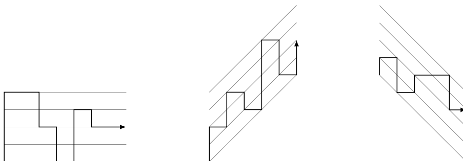
921 Figure 7: Some models of self-avoiding walks are encoded by partially directed lattice paths 922 avoiding a pattern (see [6]).
