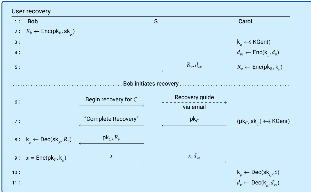
Figure 23: An overview of what keys are available to whom and when to support data recovery.
