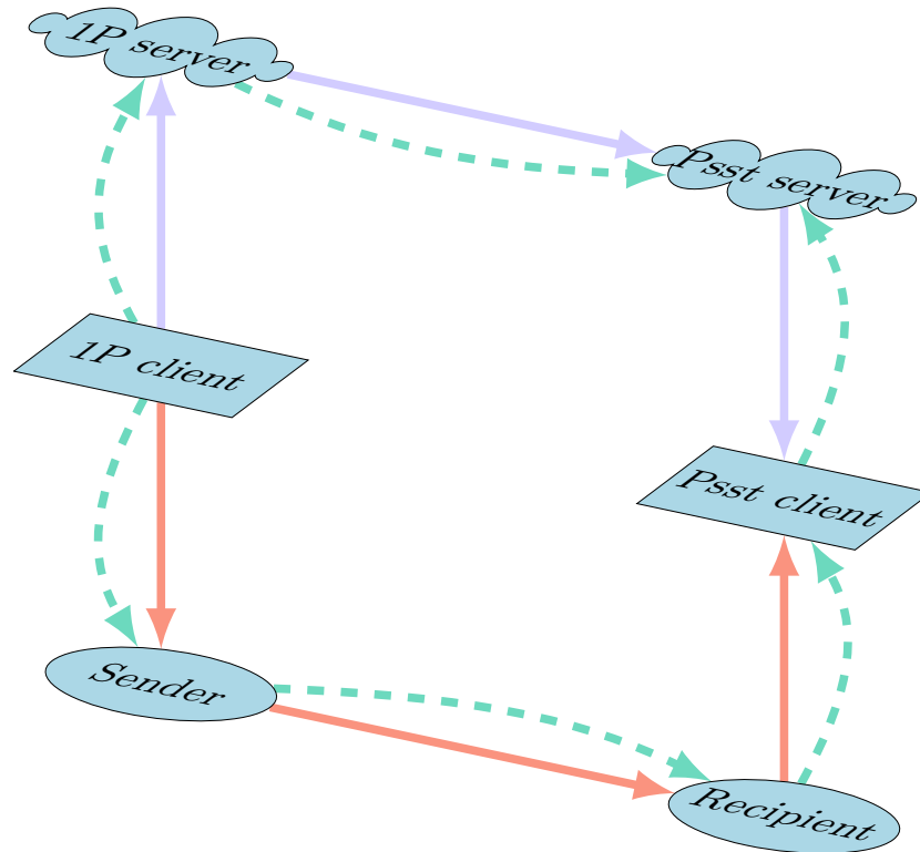
Figure 10: Psst share, key, and token flow. The solid purple arrows show the flow of the encrypted item, the solid red arrows show the flow of the encryption key, and the dashed green arrows show the flow to the retrieval token.
