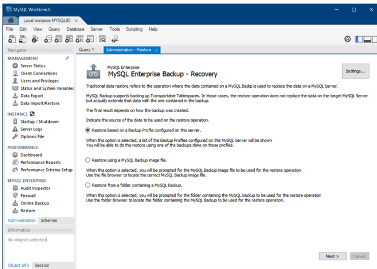
Figure 6.29 Workbench: MySQL Enterprise Backup - Recovery
