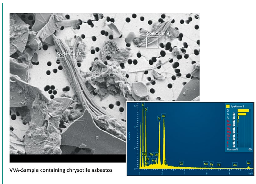
Figure 1: Scanning electron microscope (SEM) image of the «VVA» layer suspension with bundles of elongated chrysotile fibers obtained.
