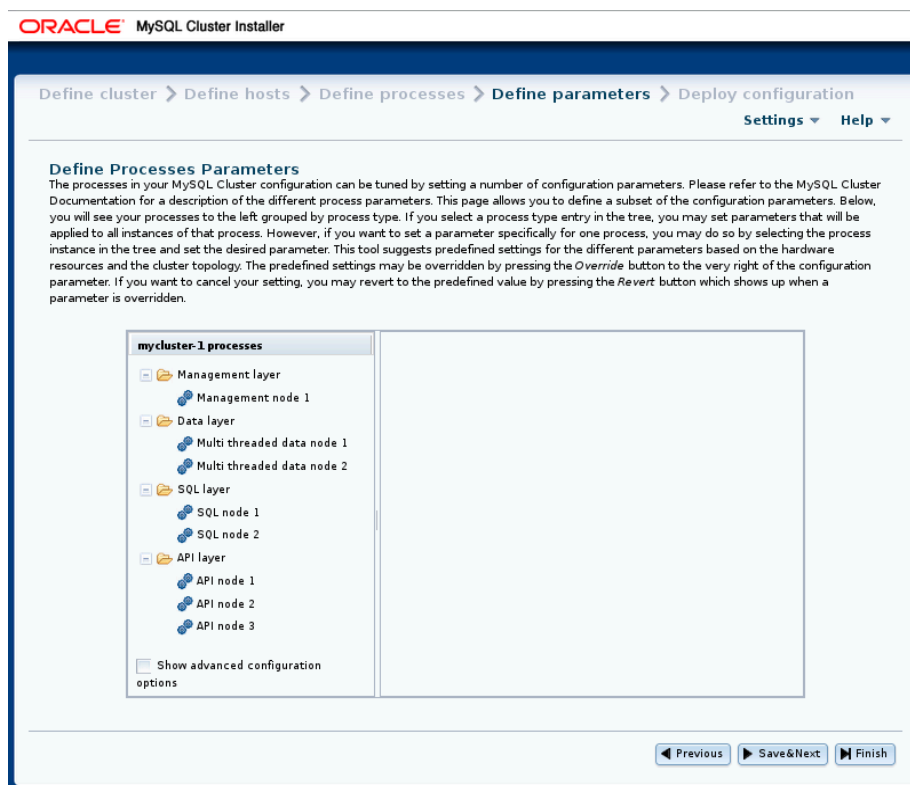
Figure 3.27 NDB Cluster Auto-Installer Define Parameters screen
