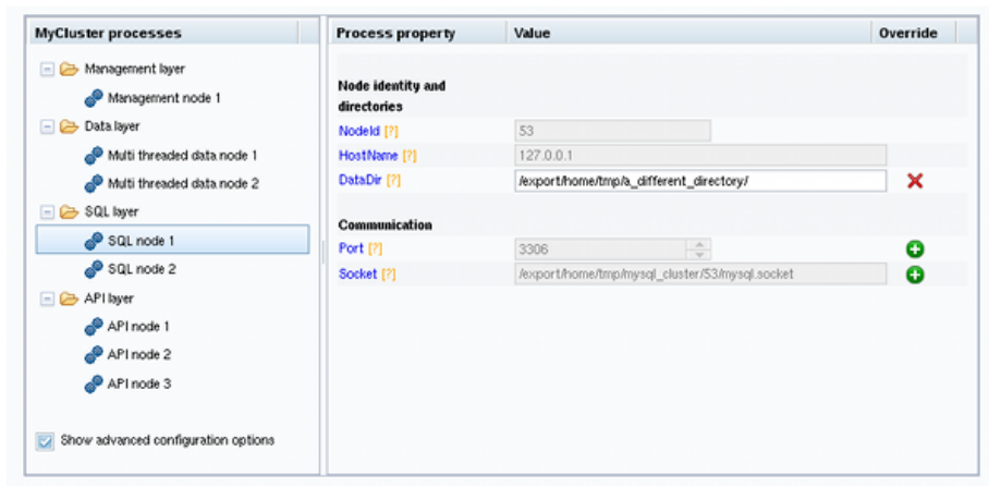
Figure 3.12 Define Attributes Detail, Overriding Attribute Default Value
