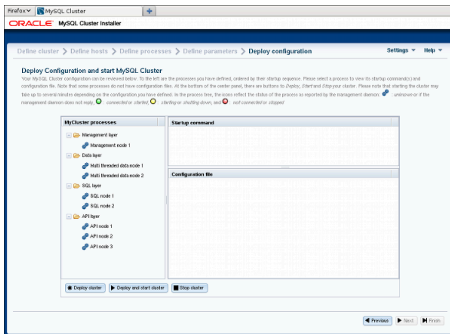
Figure 3.13 NDB Cluster Auto-Installer Deploy Cluster Configuration screen
