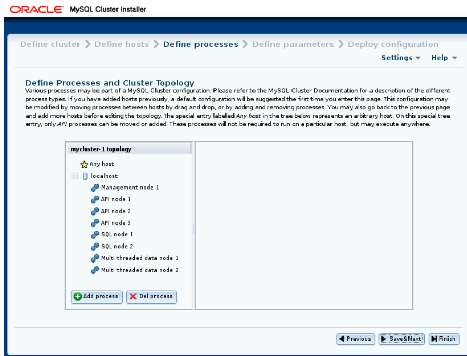
Figure 3.25 NDB Cluster Auto-Installer Define Processes dialog
