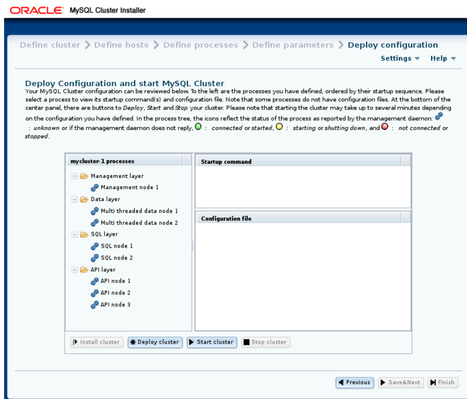
Figure 3.29 NDB Cluster Auto-Installer Deploy Configuration screen
