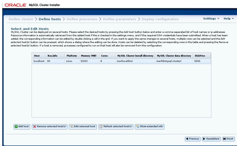
Figure 3.21 NDB Cluster Define Hosts screen, start
