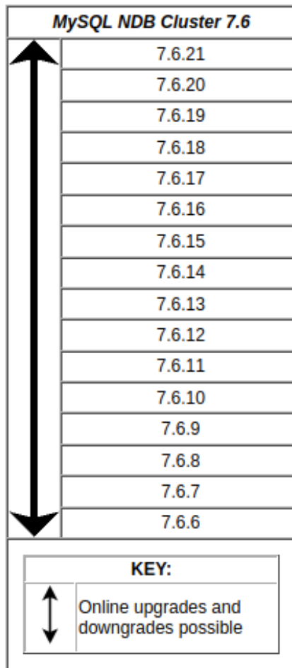
Figure 3.3 NDB Cluster Upgrade and Downgrade Compatibility, MySQL NDB Cluster 7.6
