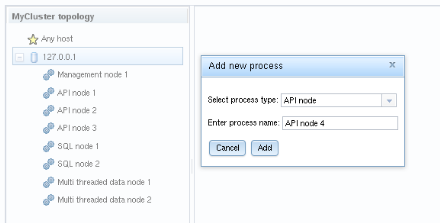
Figure 3.9 NDB Cluster Auto-Installer Add Process Dialog
