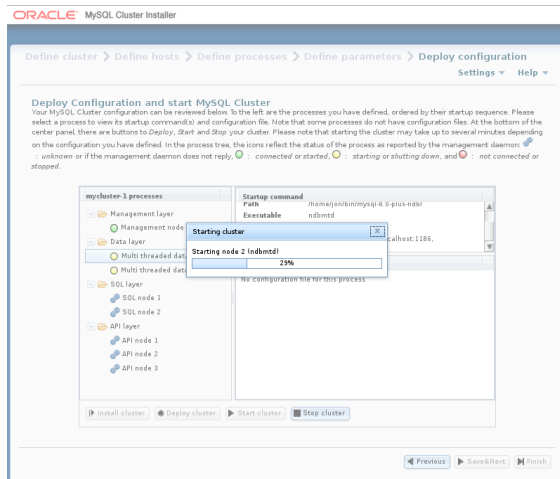
Figure 3.31 Cluster Startup Process with Progress Bar
