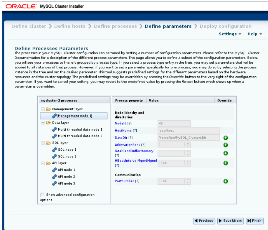
Figure 3.28 Define Parameters—Process Attributes
