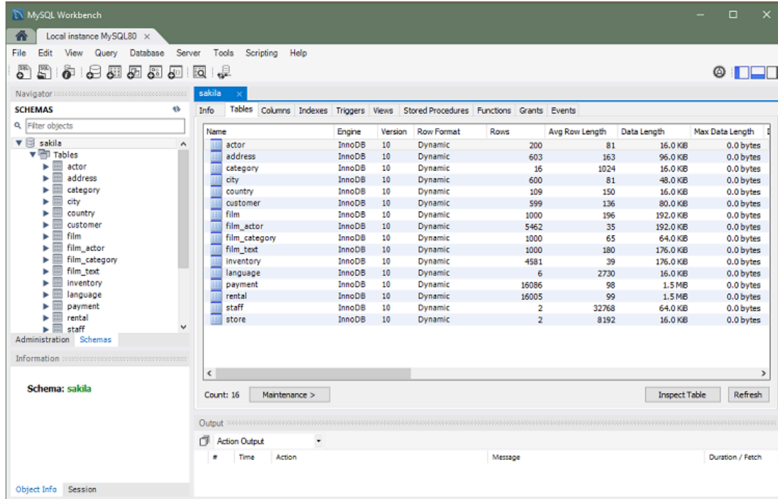
Figure 8.23 Schema Inspector
