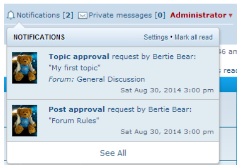
Figure 5.4. Notifications Menu
