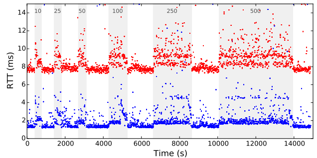
Figure 2: Delays measured from a v2 probe systematically increase when concurrent one-off traceroutes are launched on this probe.
