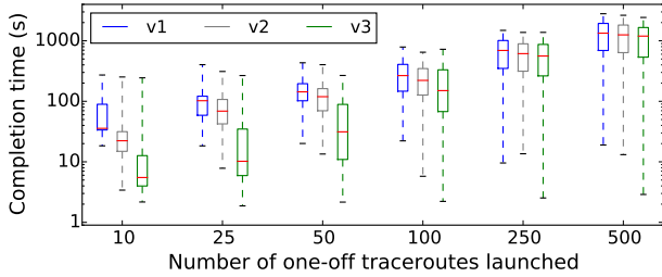
Figure 7: One-off traceroutes completion time is also impacted by concurrent measurements, independent of the hardware used. Results can be delayed by more than half an hour—making it impossible to perform synchronized experiments.
