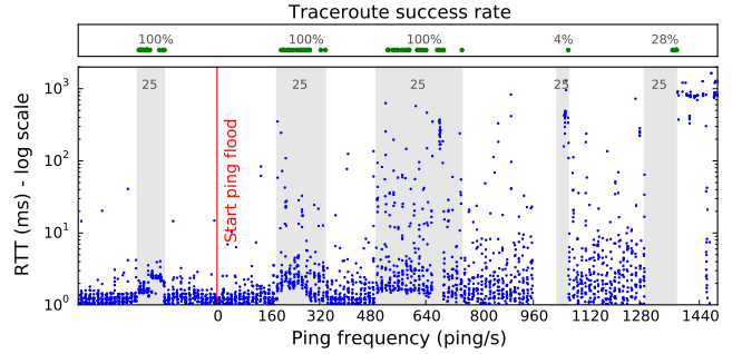
Figure 6: Increasing the source and destination load at the same time greatly increases the interference between measurements. One-off traceroutes take more time to execute, and worse, may fail. RTTs measured from the probe become higher.
