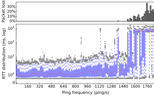
Figure 5: Delays measured towards a v2 probe increase as the pings frequency targeting this probe increases. Packet losses may appear if the ping frequency towards the probe becomes too high.
