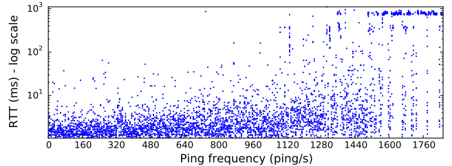
Figure 4: Delays measured from a v2 probe increase as the ping frequency targeting the probe increases.
