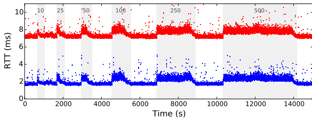
Figure 3: Delays measured towards a v2 probe systematically increase when concurrent one-off traceroutes are launched on the probe.
