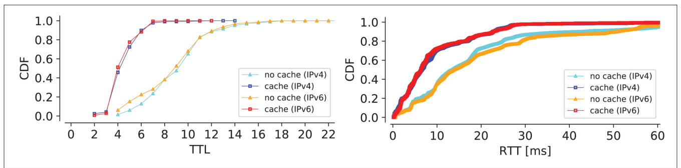
Figure 5. Comparison of path lengths (left) and latency (right) of individual IPv4 and IPv6 samples, split by cache and no-cache deployments. Caches reduce IP path lengths and latencies by up to ~50 percent.
