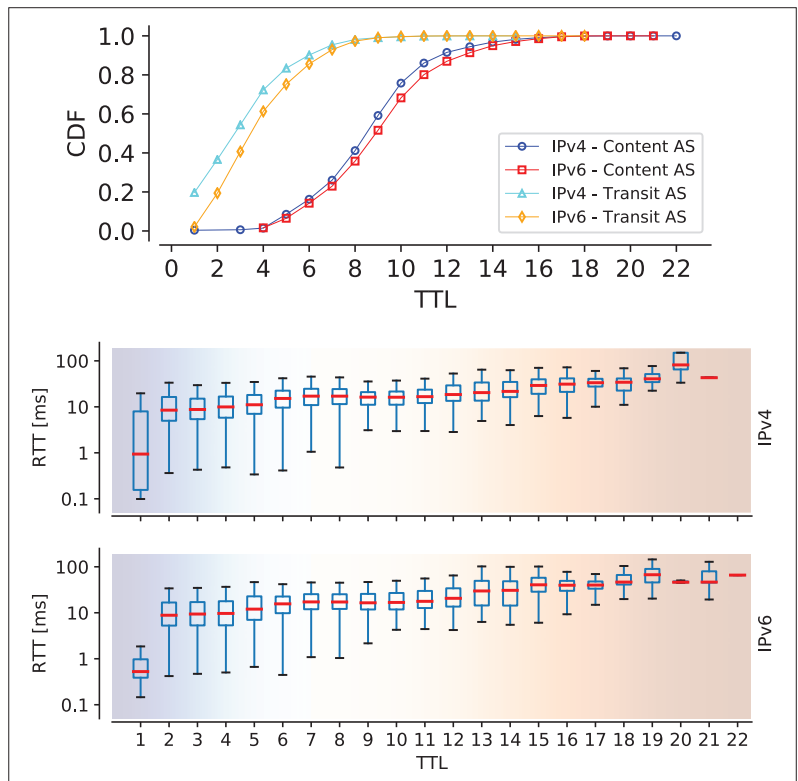
Figure 6. a) Distribution of path lengths towards intermediate IP endpoints classified by AS types. Path lengths up to 7 IP hops can serve as a heuristic to delineate the boundary of ISP networks and CDN providers. b) Boxplots of latency by path lengths over IPv4 (top) and over IPv6 (bottom) as seen from residential vantage points. The blue tone represents caches in ISP networks, while the red tone represents CDNs.
