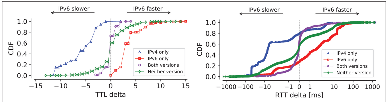
Figure 4. Distribution of deltas of TTL (left) and RTT (right) for destination pairs, classified by cache presence for IPv4 and IPv6: (1) IPv4 only; (2) IPv6 only; (3) Cache present for both address families; (4) No cache present for either address family. Latency and path length distributions shift away from congruency when a cache was available over one address family only. Latency and path lengths are comparable between address families in situations when caches were dual-stacked.
