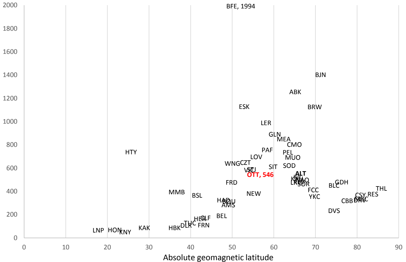
Maximum one-minute change in horizontal magnetic field, March 13, 1989 (nanotesla)
