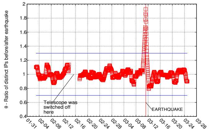
Figure 10: Ratio of number of IP addresses reaching the UCSD darknet in two successive 24-hour periods (before vs after the given data point) from networks within a \rho_{max} = 304 \text{ km} range from the Tohoku earthquake's epicenter. Although we use a different distance threshold than for the \theta values in the Christchurch plot in Figure 9, there is a similar breakout above a \theta ratio of 1.3 exactly when the earthquake strikes.
