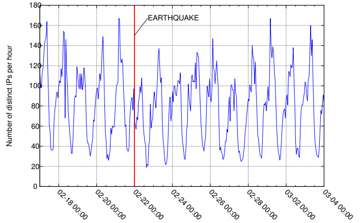
Figure 7: Rate of unique source IP addresses found in unsolicited traffic reaching the UCSD network telescope from networks geolocated within a \rho_{max} = 20\text{ km} range from the Christchurch earthquake epicenter. The rate of distinct IPs per hour drops immediately after the earthquake. Peaks before the earthquake were above 140-160 IPs/hour on weekdays (weekend is on 19-20 February), while the first peak after the earthquake is slightly above 100 IPs/hour. Levels remain lower for several days, consistent with the slow restoration of power in the area.
