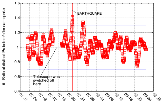
Figure 9: Ratio of number of unique IP addresses reaching the UCSD darknet in two successive 24-hour periods (before vs after the given data point) from networks within a \rho_{max} = 20 \text{ km} range from the Christchurch earthquake's epicenter. We plot this \theta value over this two-month period, using two sliding 24-hour windows before and after each point plotted. The anomalous breakout above the 1.3 upper bound of \theta coincides with the earthquake strike, and represents a large (about 30%) drop in the number of IP addresses reaching the UCSD darknet. The corresponding drop is also visible, although less obvious, in Figure 7.
