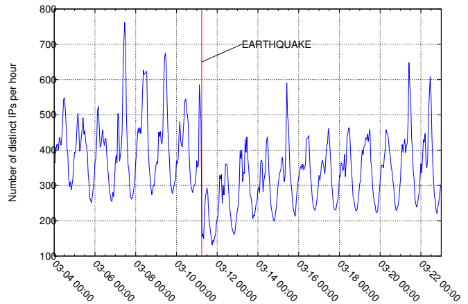
Figure 8: Rate of unique source IP addresses found in unsolicited traffic reaching the UCSD network telescope from networks geolocated within \rho_{max} = 304\text{ km} of the Tohoku earthquake epicenter. The rate of distinct IPs per hour shows a considerable drop after the earthquake which does not return to previous levels even after several days.
