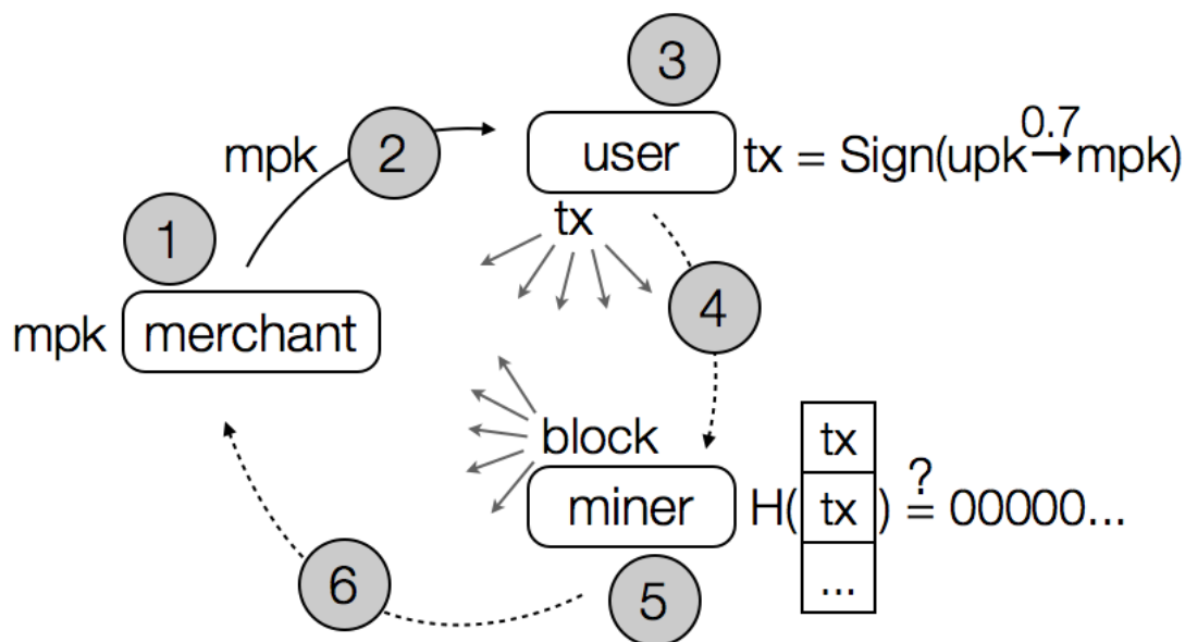
Figure 4.1. How a Bitcoin transaction works. In this example, a user wants to send 0.7 bitcoins as payment to a merchant. In (1), the merchant generates or picks an existing public key mpk , and in (2) it sends this public key to the user. In (3), by creating a digital signature, the user forms the transaction tx to transfer the 0.7 bitcoins from his public key upk to the merchant's address mpk . In (4), the user broadcasts this transaction to his peers, which (if the transaction is valid) allows it to flood the network. In this way, a miner learns about his transaction. In (5), the miner works to incorporate this and other transactions into a block by checking if their hash is within some target range. In (6), the miner broadcasts this block to her peers, which (if the block is valid) allows it to flood the network. In this way, the merchant learns that the transaction has been accepted into the global block chain, and has thus received the user's payment.
