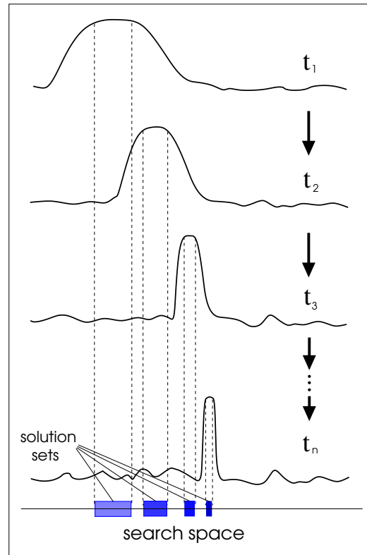
Figure 5.3: Incremental fitness landscapes. The figure illustrates, for a 1-dimensional search space, how incremental evolution works by gradually reshaping the fitness landscape to guide the population toward a solution to the goal task.
