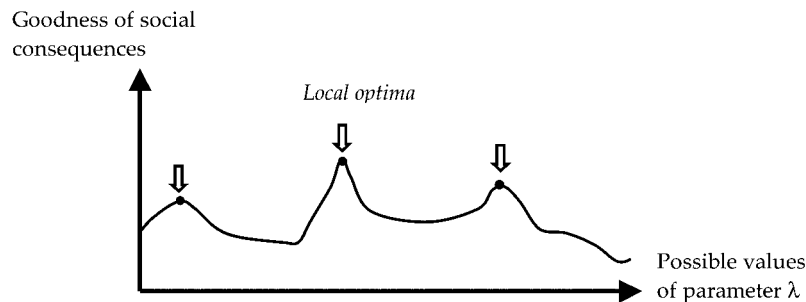
FIG. 1.—Only the points indicated with arrows are local optima. Typically, only a few points will be local optima, and most points will be such that a small shift in \lambda in the appropriate direction will increase the goodness of the social consequences.
