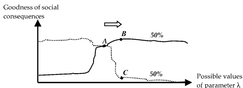
FIG. 2.—There is uncertainty whether the goodness of social consequences of a given value of a parameter \lambda is represented by the solid or the dotted line. A society that is currently in state A is not at a local optimum but may nevertheless resist a small shift in the parameter \lambda because of the risk that it would bring about state C rather than state B.
