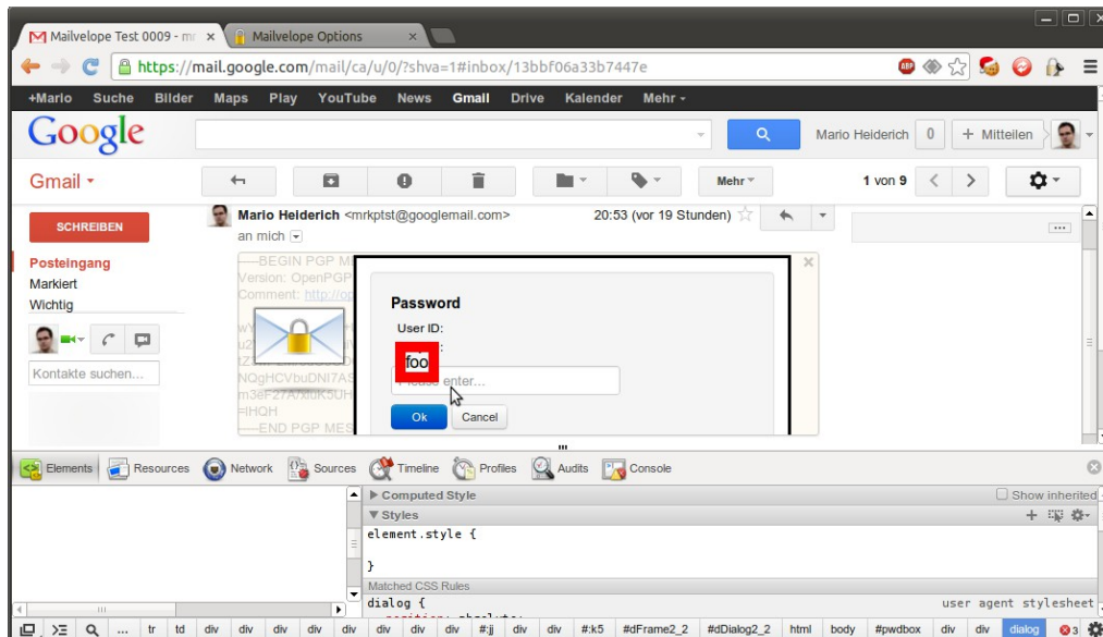
Figure B4: Example injection overlapping the encryption key password field
