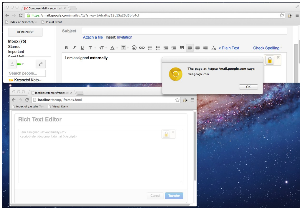
Figure C: Externally embedded RTE used to trigger XSS in webmail provider document
