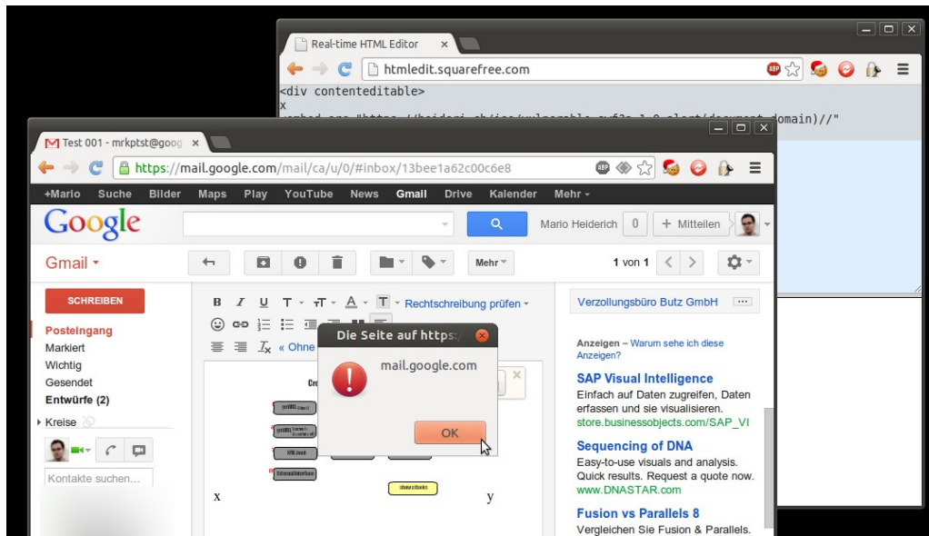
Figure E: Example for cross-domain drag&drop XSS based on insuff. RTE protection
