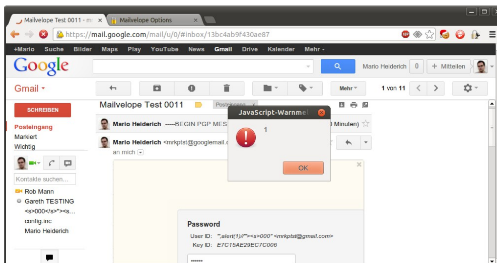
Figure B3: Executing arbitrary JavaScript on about:blank via object / embed
