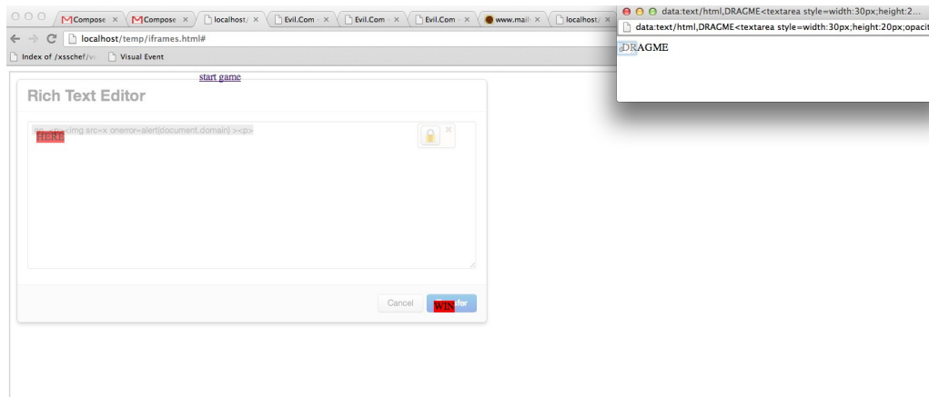
Figure D: UI redressing Rich Text Editor
