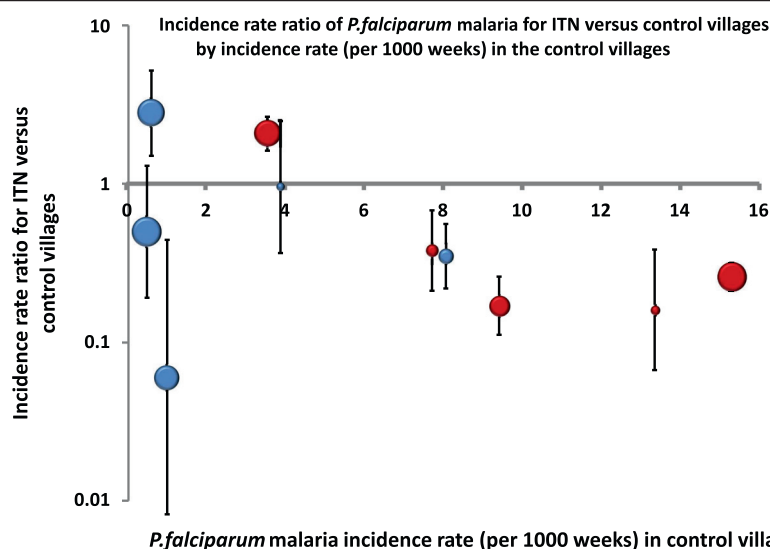
Figure 3 Incidence rate ratio of P.falciparum for ITN versus control (NN) villages by incidence rate (per 1000 weeks) in the control villages.
