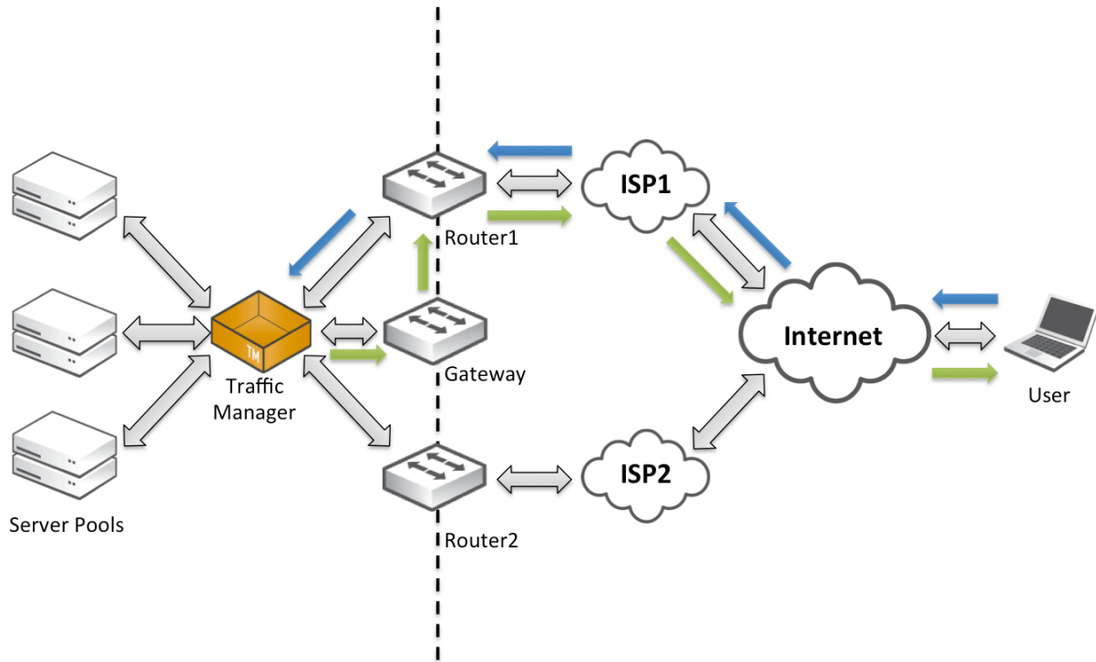
Fig 67. Employing a gateway router to perform connection tracking
