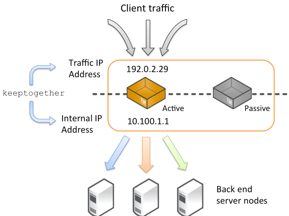
Fig 4. The Traffic IP and Internal IP are bound together in a traffic IP group
