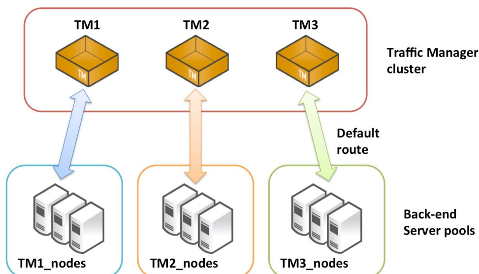
Fig 5. Partitioning your servers into Traffic Manager specific pools
