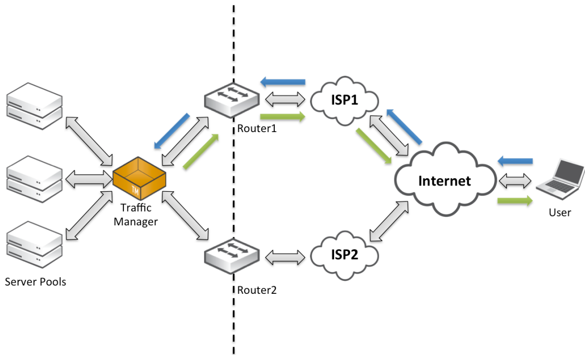
Fig 68. Return path routing is enabled
