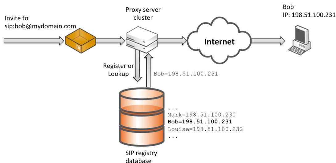
Fig 37. Detail of how an IP phone call using SIP would work with a Traffic Manager
