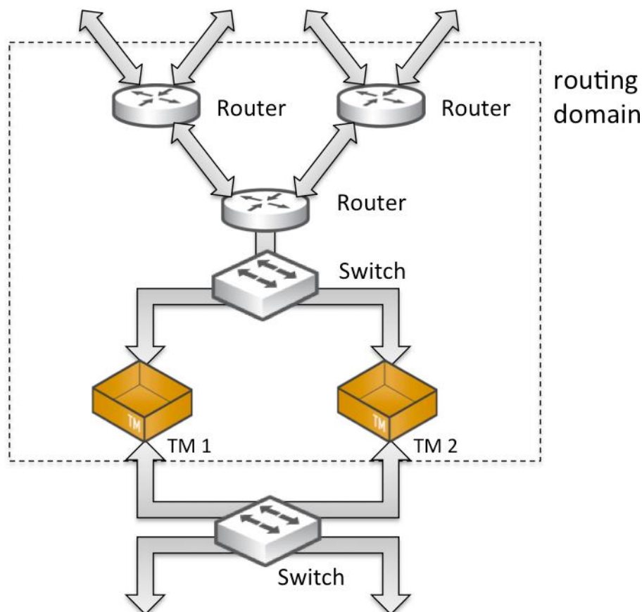
Fig 6. Advertising traffic IP addresses using RHI
