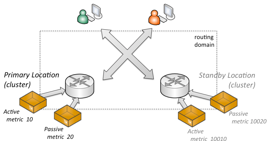
Fig 7. A dual datacenter deployment with RHI
