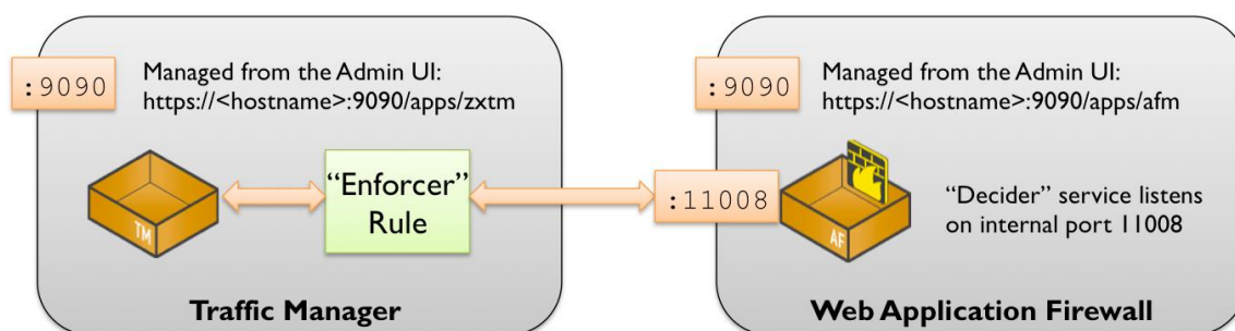
Fig 26. The Traffic Manager's Enforcer TrafficScript rule forwards requests to the default local port 11008 for inspection by the Decider service. The Decider returns a "Permit" or "Deny" decision and the Enforcer rule applies the decision.
