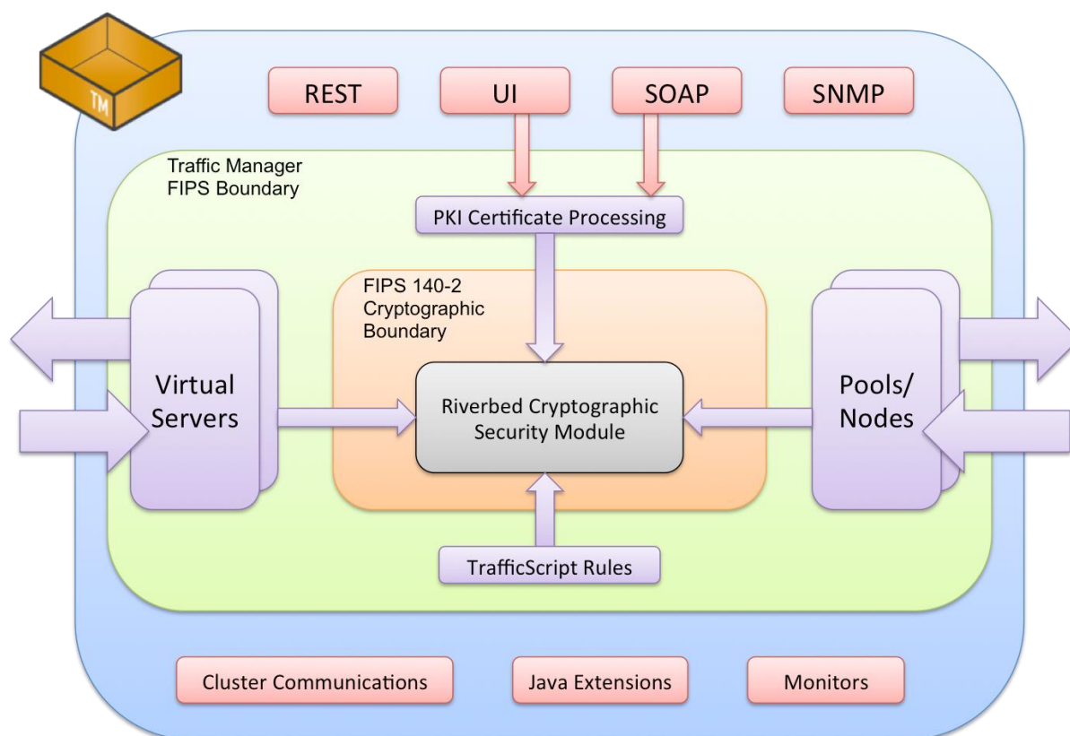
Fig 82. The Traffic Manager FIPS boundary
