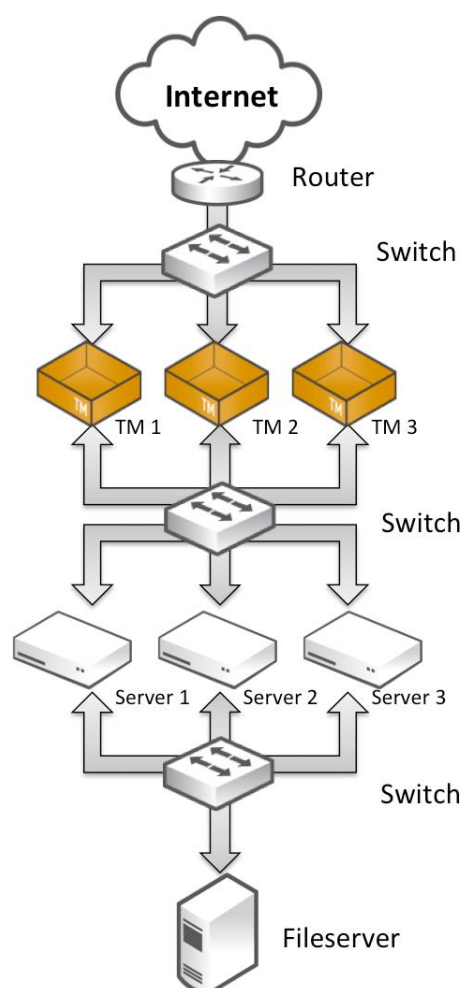
Fig 2. Fault-tolerant network with a cluster of Traffic Manager units serving back-end nodes
