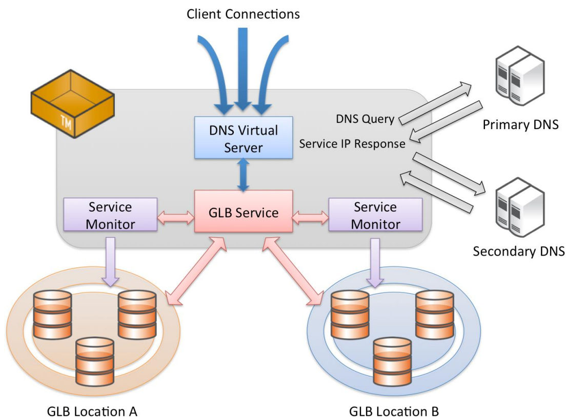
Fig 81. The components of a Traffic Manager GLB deployment
