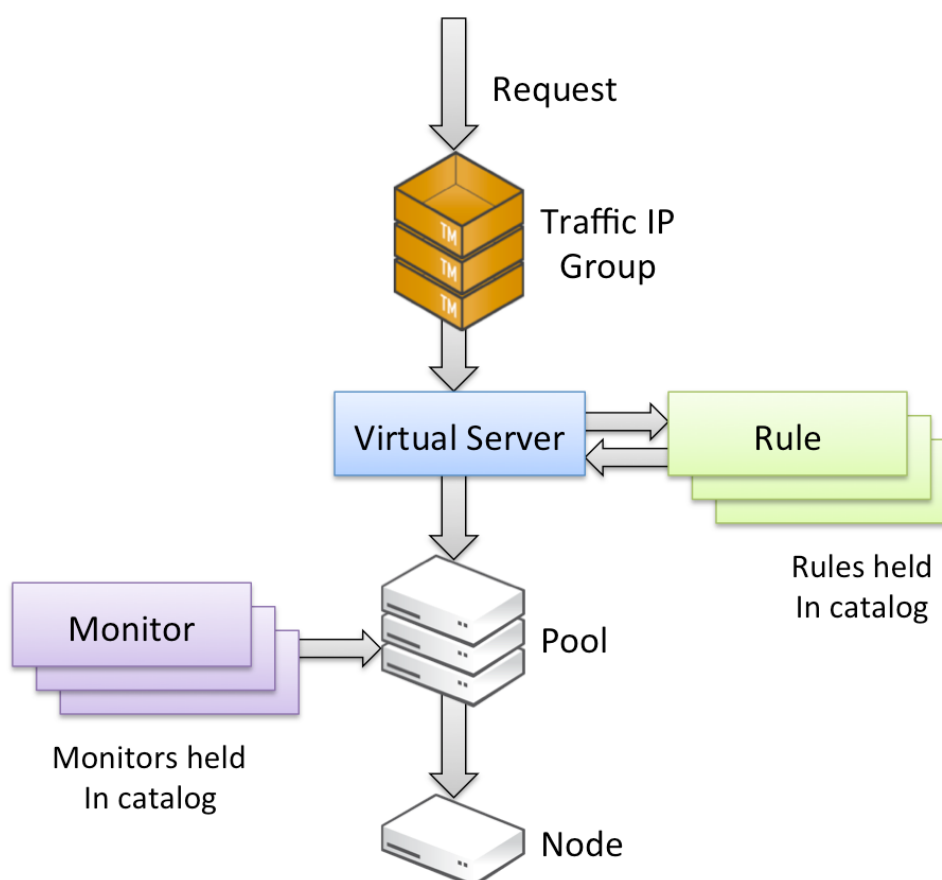
Fig 8. A basic Traffic Manager configuration
