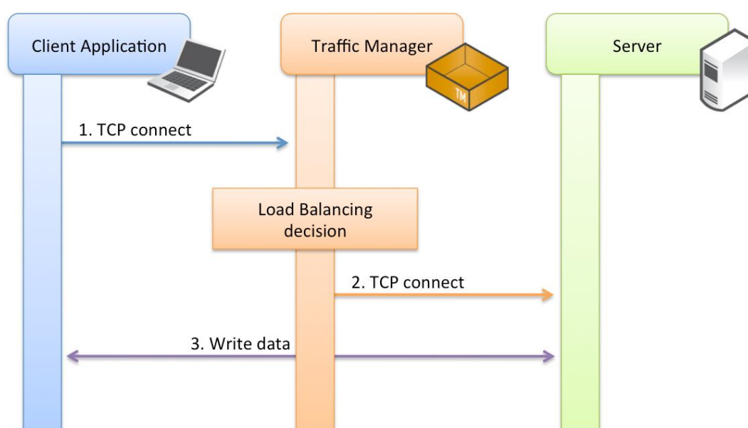
Fig 34. Load balancing with generic streaming protocols
