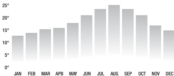
Average air temperature (Celsius)
