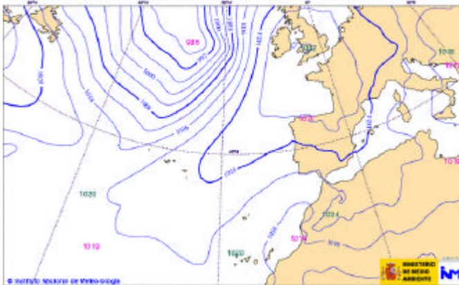
Surface chart (isobars and precipitation forecasted at 14:00 LST)
