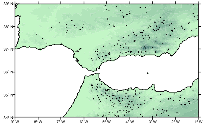
Surface analysis 09-12-2003 at 06:00 utc (07:00 LST)
