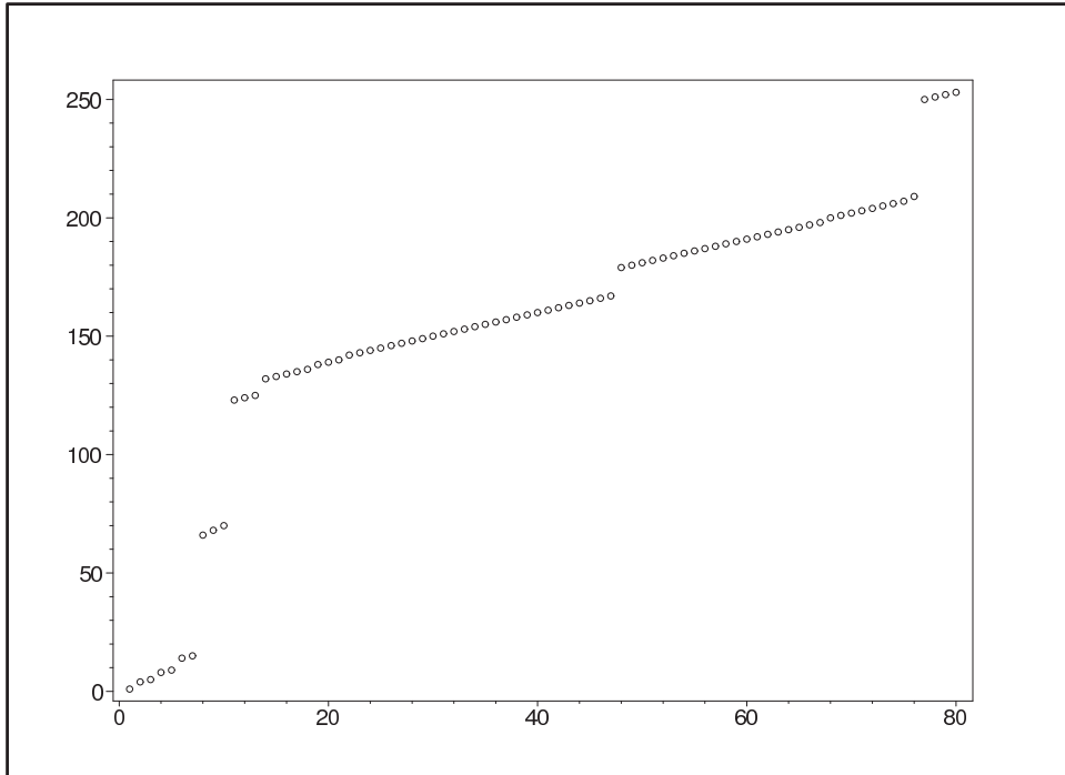
Figure 4: Scatter-plot of lower bounds on \mu(n) , the record for a starting sequence of n 2's and 3's. Entries for n \leq 47 are known to be exact (and we conjecture the other entries are exact).
