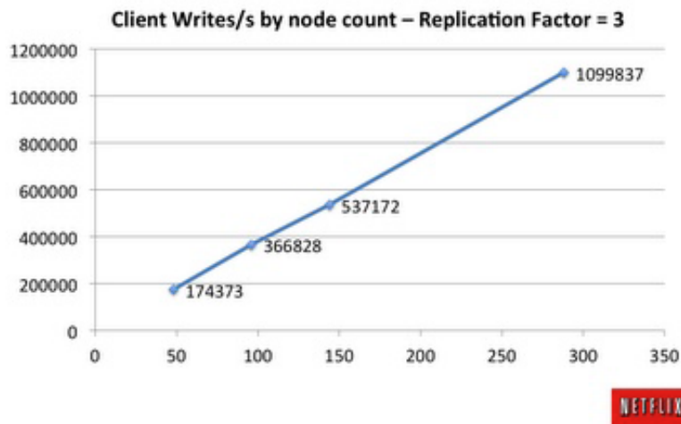
Figure 3: Performance results from Netflix's cloud benchmark of Cassandra
