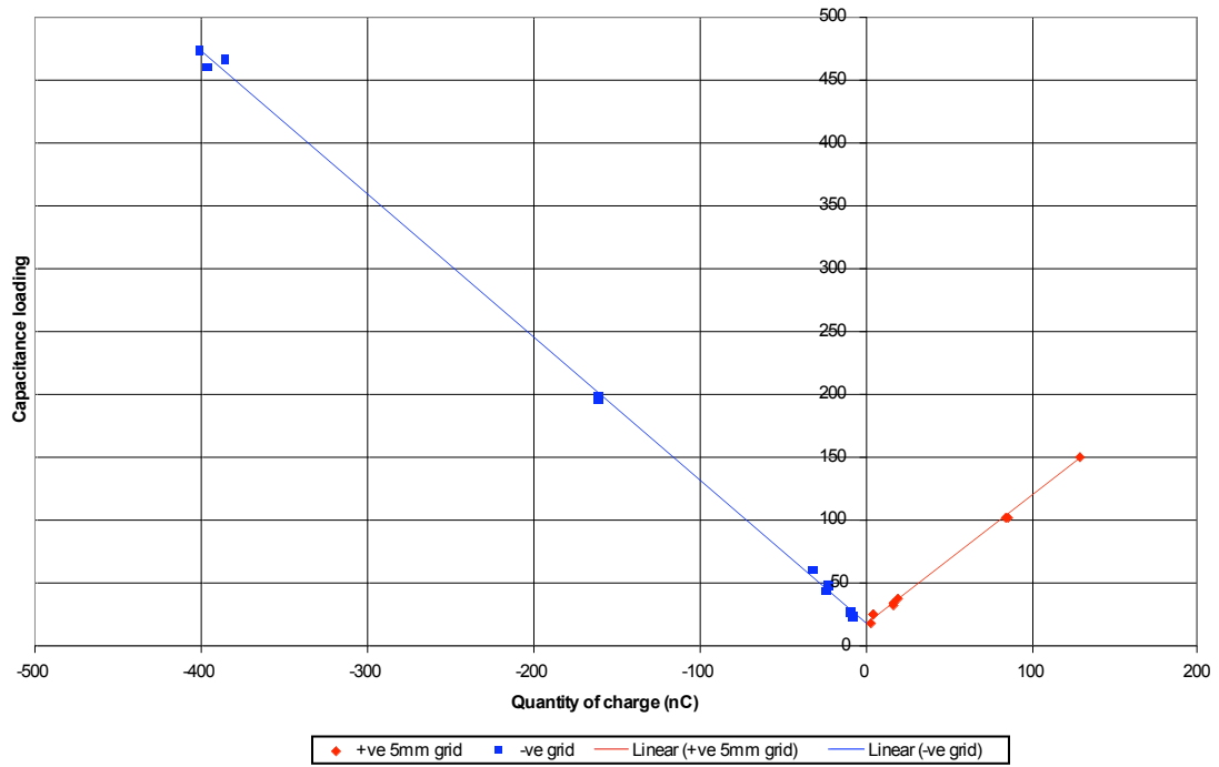
Variation of capacitance loading with quantity of charge - 5mm grid conductive thread
