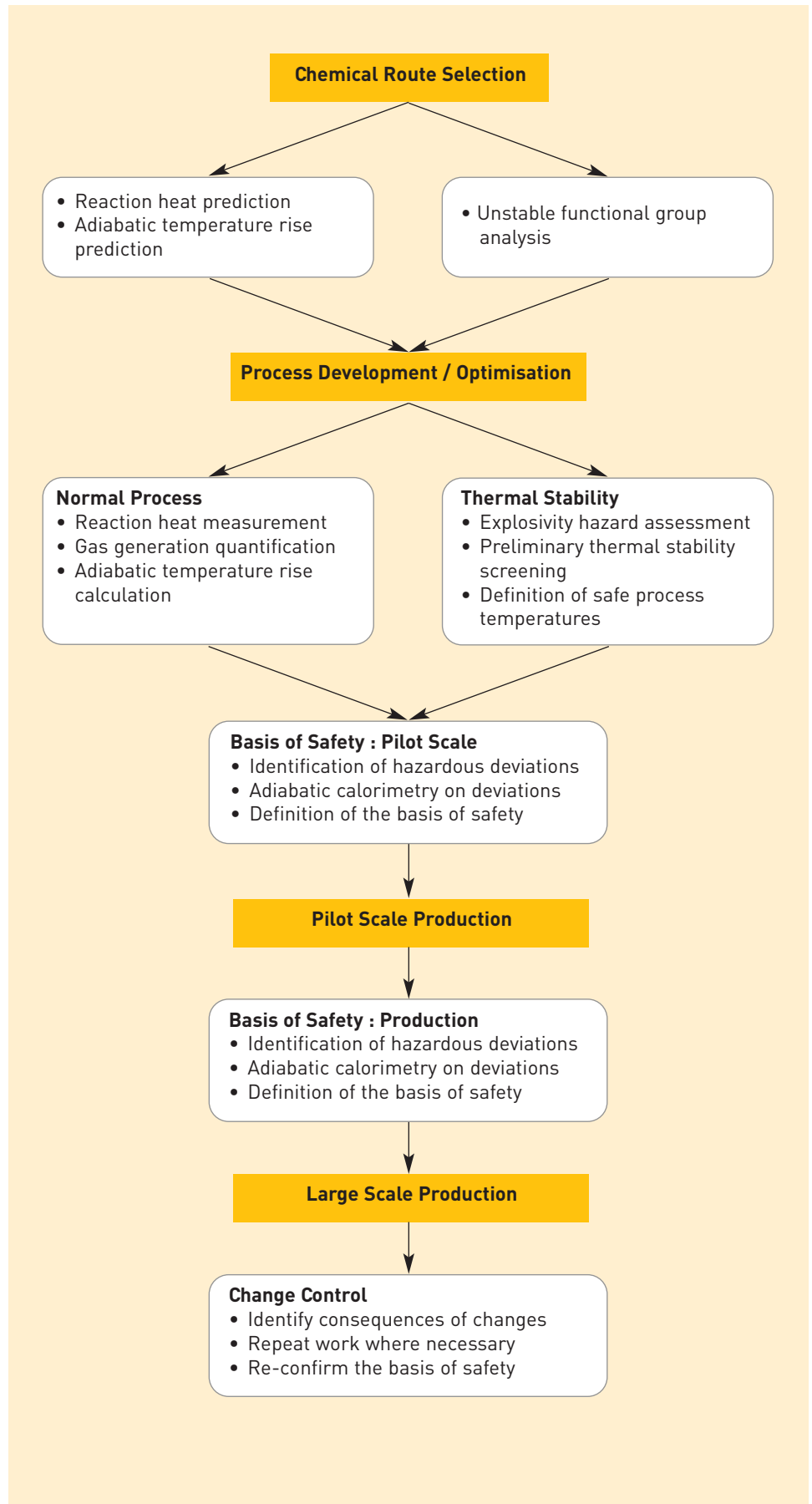
Figure 1: A Strategy for Reaction Hazard Evaluation
