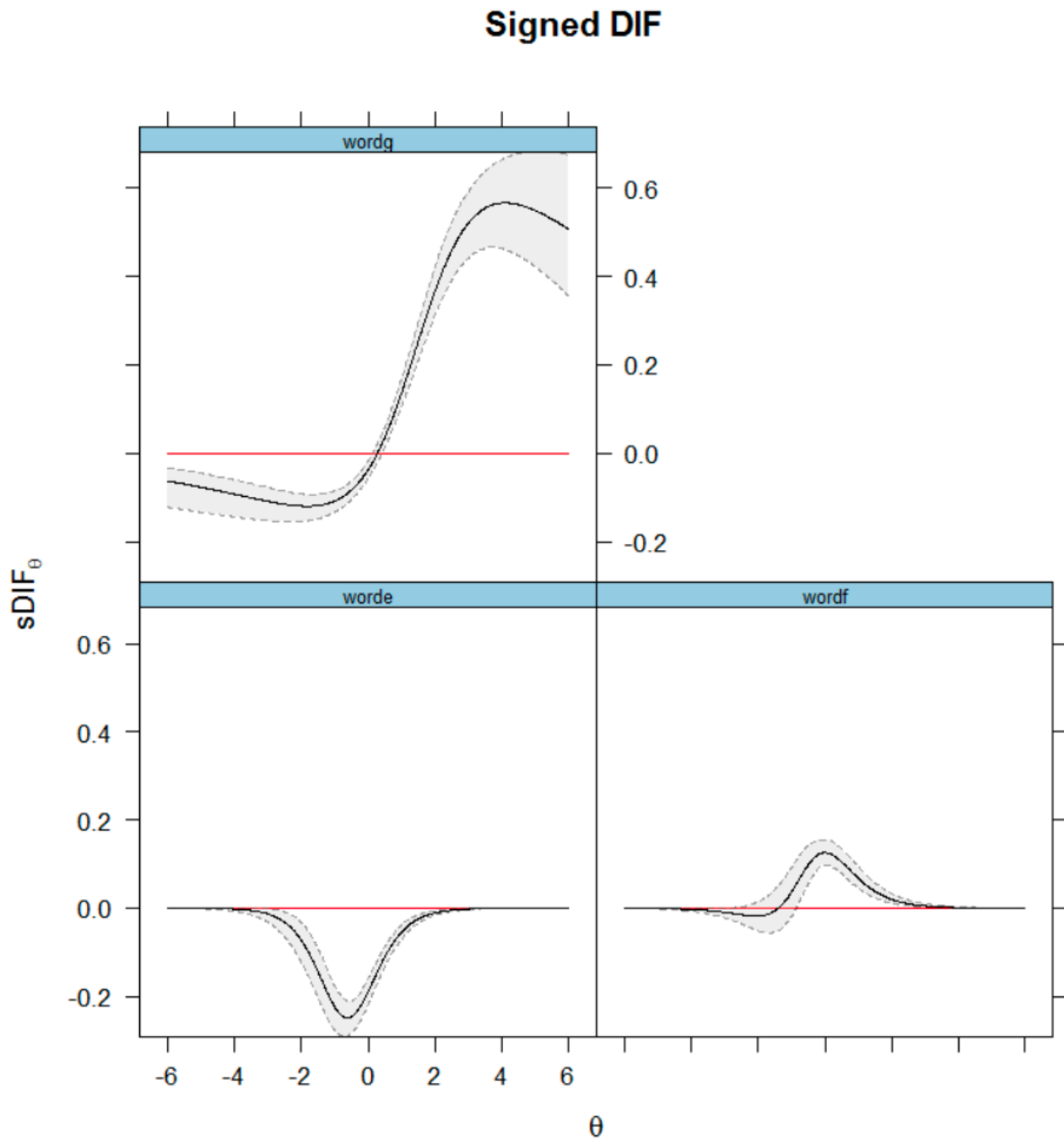
Figure 1: Differential Response Functioning Plots for Racial Groups. The X axis shows the latent score ( \theta ) distribution while the Y axis shows the signed DRF for each DIF item.
