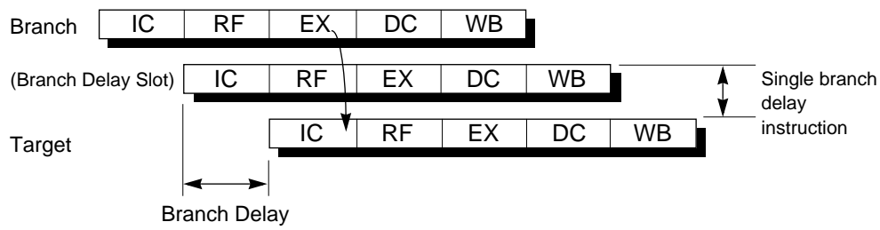
Figure 4-4 Branch Delay
