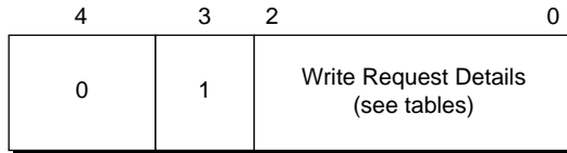
Figure 12-34 Write Request SysCmd(4:0) Bus Bit Definition
