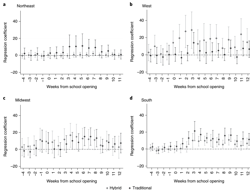
Fig. 3 | Adjusted absolute difference between SARS-CoV-2 cases in counties with hybrid and traditional school modes relative to virtual for each week, with week 0 being the week when school started for each county, stratified by region. a–d. Results were generated from multivariate Poisson regressions with robust s.e. for the Northeast (a), West (b), Midwest (c) and South (d). The black markers indicate traditional school mode and the gray markers indicate hybrid school mode. The whiskers for each marker depict the upper and lower bounds of the 95% CI ( n = 1,512 for the Northeast, 648 for the West, 1,887 for the Midwest and 3,110 for the South). Google mobility data were not available for week 12 following school opening in the Northeast, thus results are presented for the 11 weeks following school opening in that region (a).
