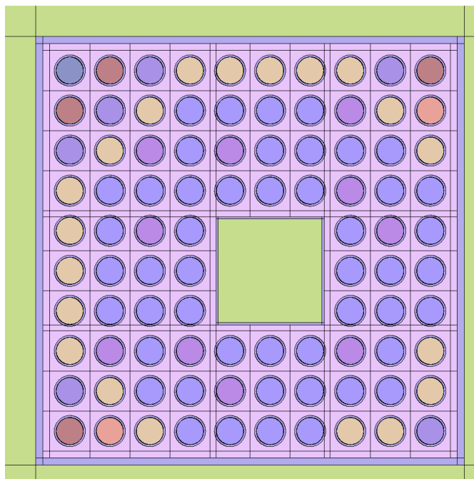
Figure 3.7: A 10x10 BWR fuel fuel assembly with 7 pin types and an asymmetrically positioned moderator channel.
