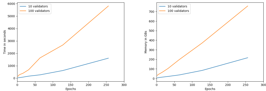
Fig. 6.1: Proving time and peak memory consumption over BW6-761.
