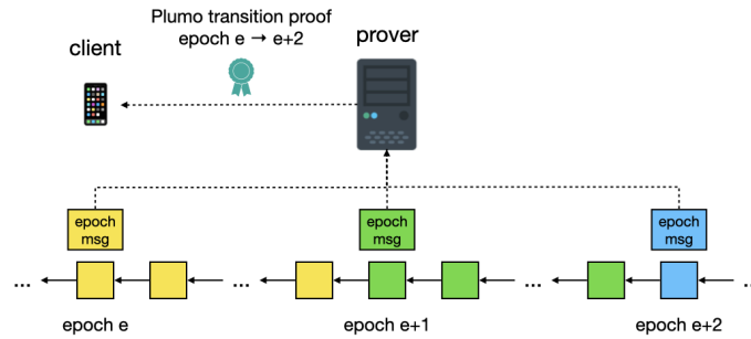
Fig. 2.1: Plumo architecture overview. In practice, our proofs cover 120 epochs.
