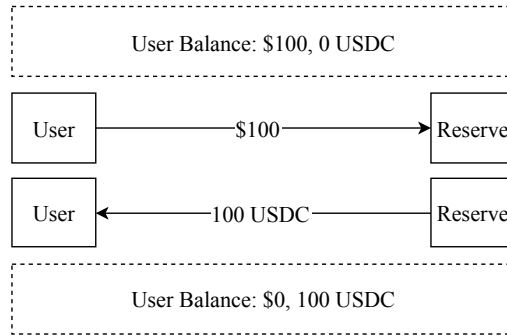
Fig. A1. Reserve of Pegged Asset (ex. USDC)
