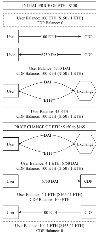
Fig. A4. Leveraged Loans (ex. Dai)
