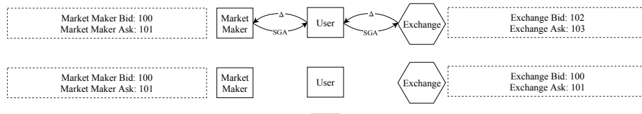
Fig. A2. Algorithmic (ex. Saga)
