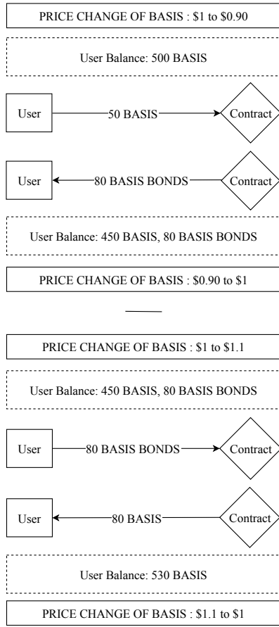
Fig. A3. Dual Coin (ex. Basis)
