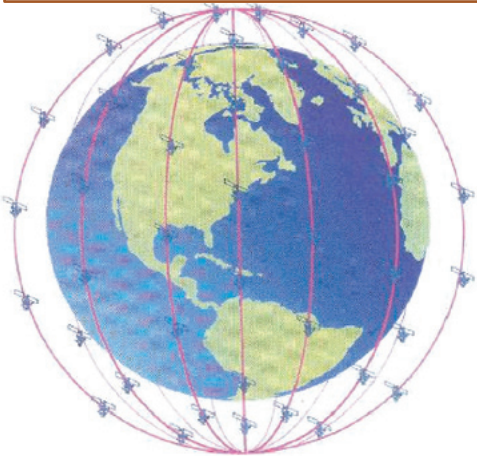
Iridium Constellation 6 rings x 11 platforms
