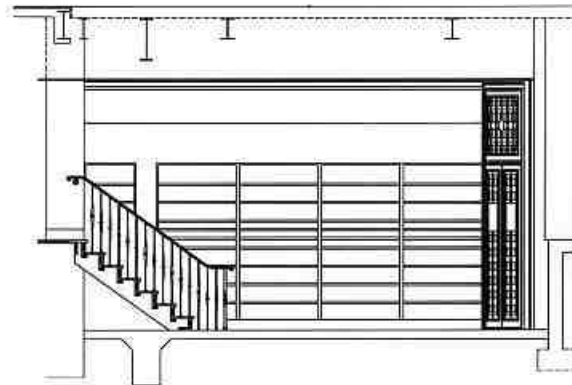
4 EAST ELEVATION 1/2" = 1'-0"
