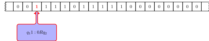
FIGURE 4: The computation of 3 + 4 by T_{Add_2}
