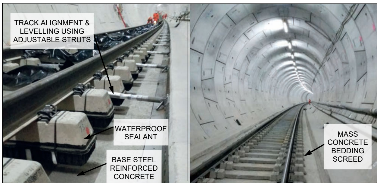
Figure A6.2 Key elements of the booted track tie system
