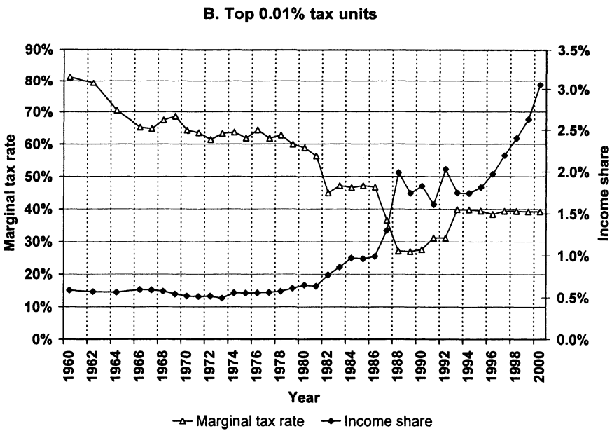
FIGURE 5. Tax Rates and Income Shares for the Top Groups
