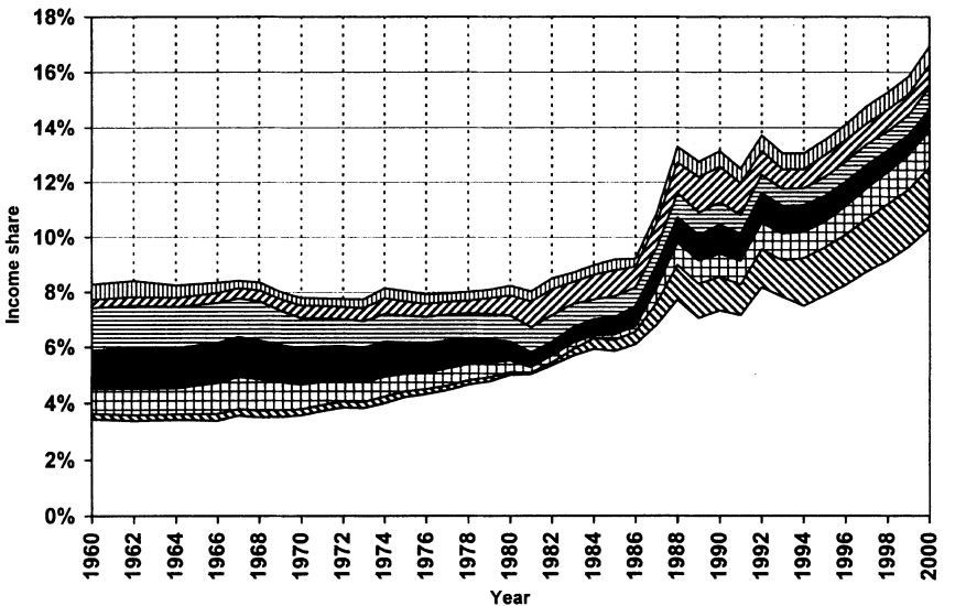
FIGURE 7. The Top 1% Income Share and Composition, 1960–2000
