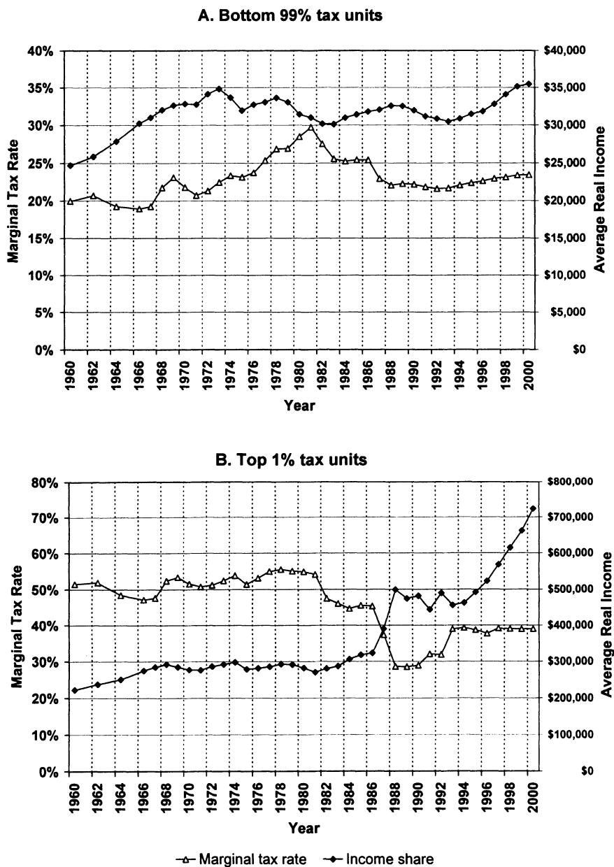
FIGURE 2. Marginal Tax Rates and Average Real Incomes for the Bottom 99% and the Top 1%
