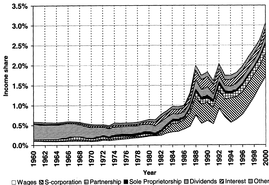
FIGURE 8. The Top 0.01% Income Share and Composition, 1960–2000
