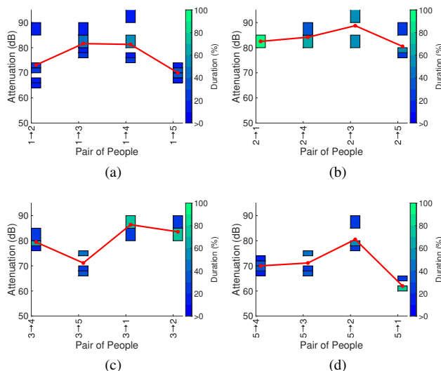
Fig. 4: Attenuation durations reported by GAEN API on completion of the second lower deck test (with the same participants as in the first test, but with their seating positions swapped about). In (d) person 5 is using a Samsung Galaxy A10 rather than a Google Pixel 2.
