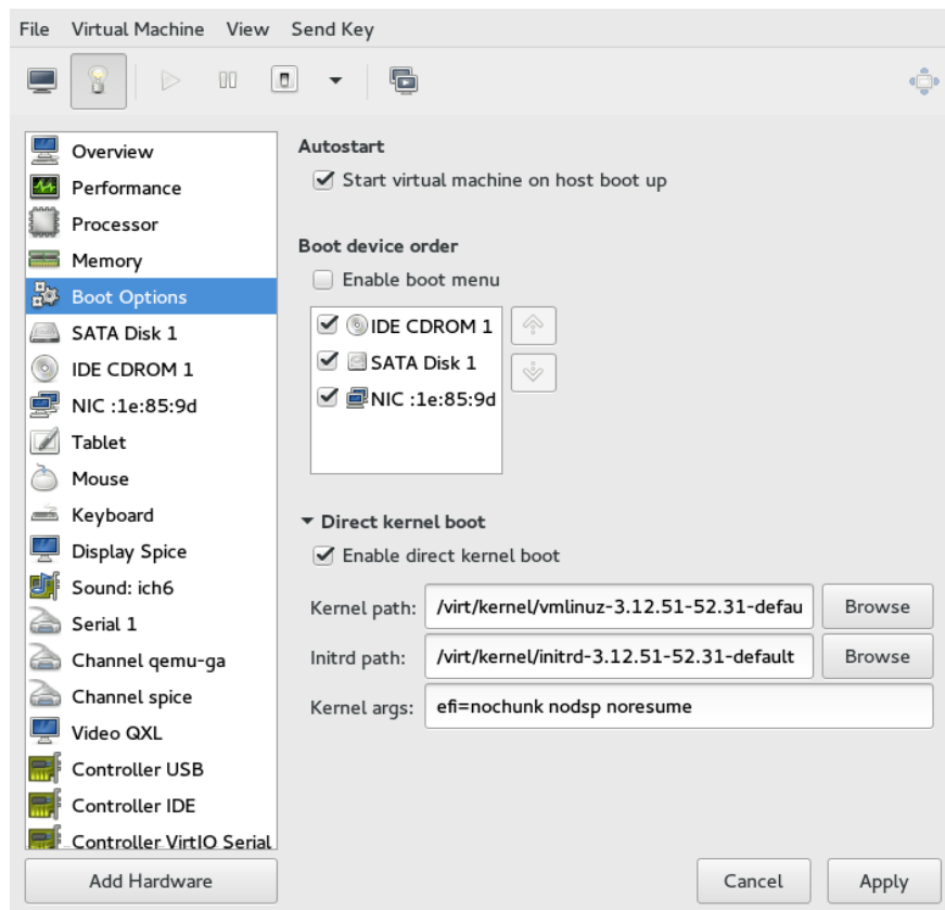
FIGURE 13.8: BOOT OPTIONS
