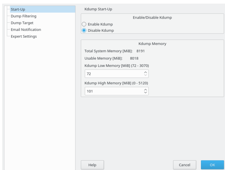
FIGURE 17.1: YAST KDUMP MODULE: START-UP PAGE
