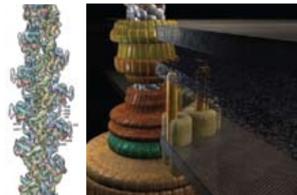
Structure of F-actin and Flagellar Motor
