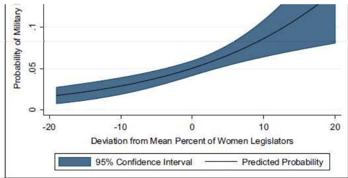
Figure 5. Predicted probabilities of humanitarian interventions, 1946–2003.
