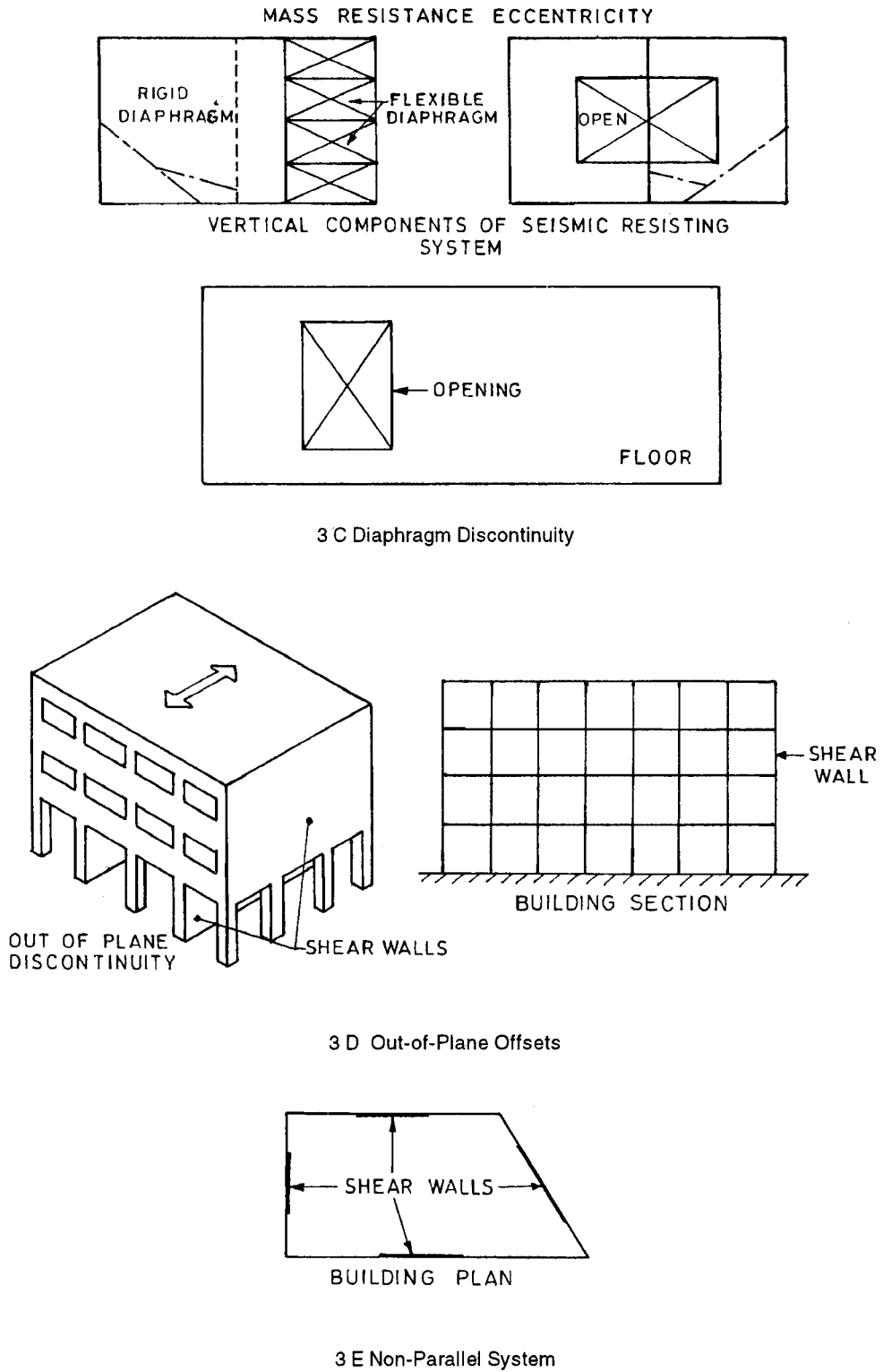
FIG. 3 PLAN IRREGULARITIES
