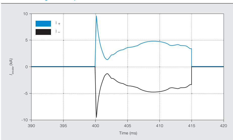
6 Currents flowing in the two poles of the circuit breaker
