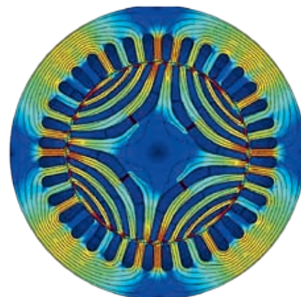
1b The rotor is not aligned with the magnetic field, and (counter-clockwise) torque is produced.
