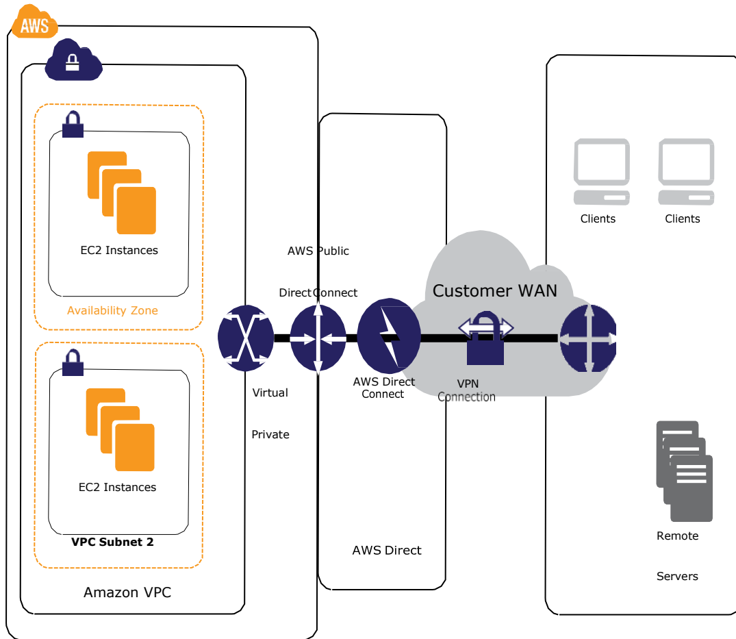
AWS Direct Connect and VPN
