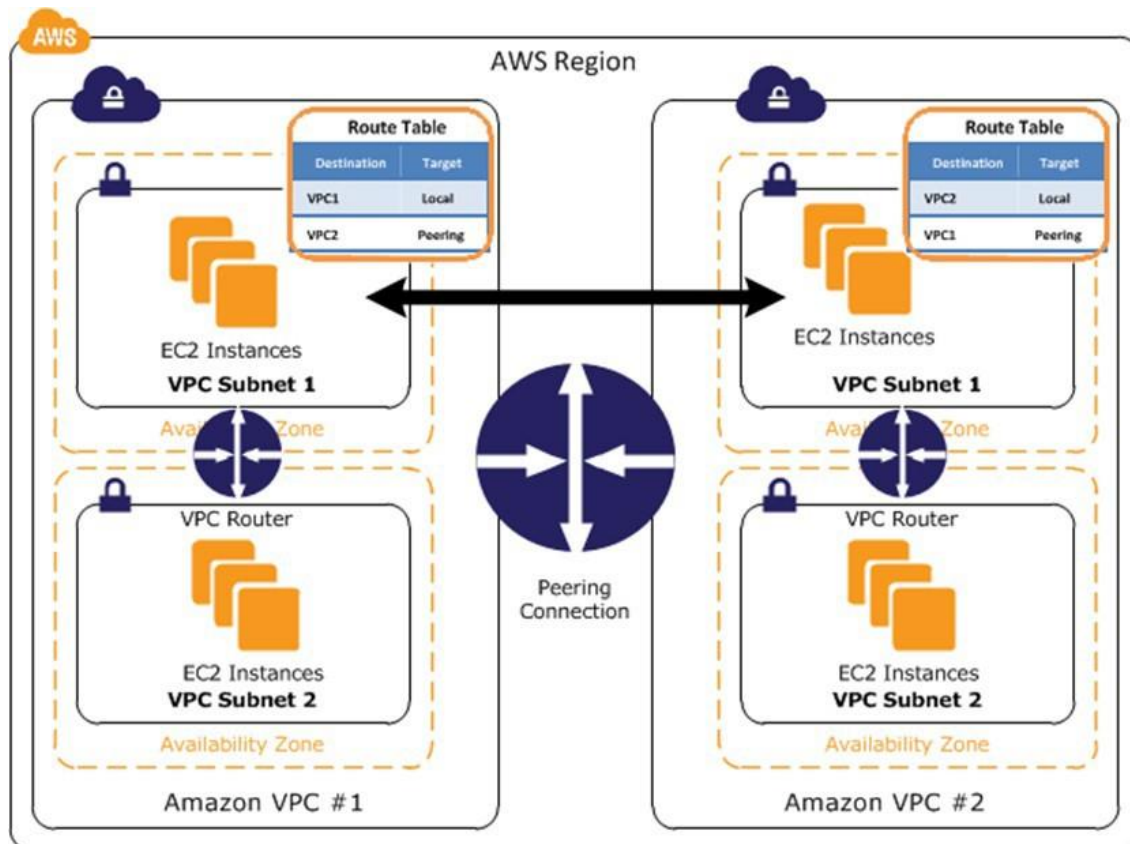
VPC-to-VPC peering
