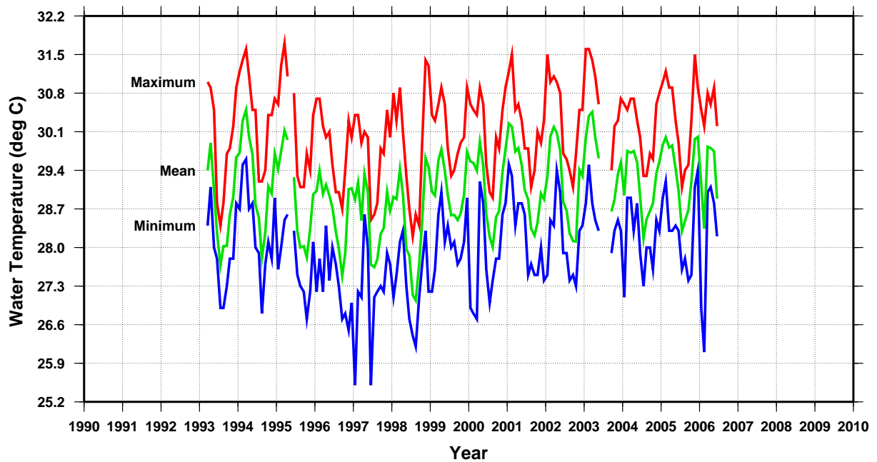
Monthly water temperature at Apia SEAFRAME gauge
