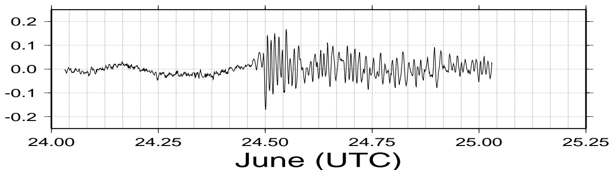
Figure 12. The non-tidal sea level record (m) at Samoa in June 2001 following a tsunamigenic earthquake off Peru.
