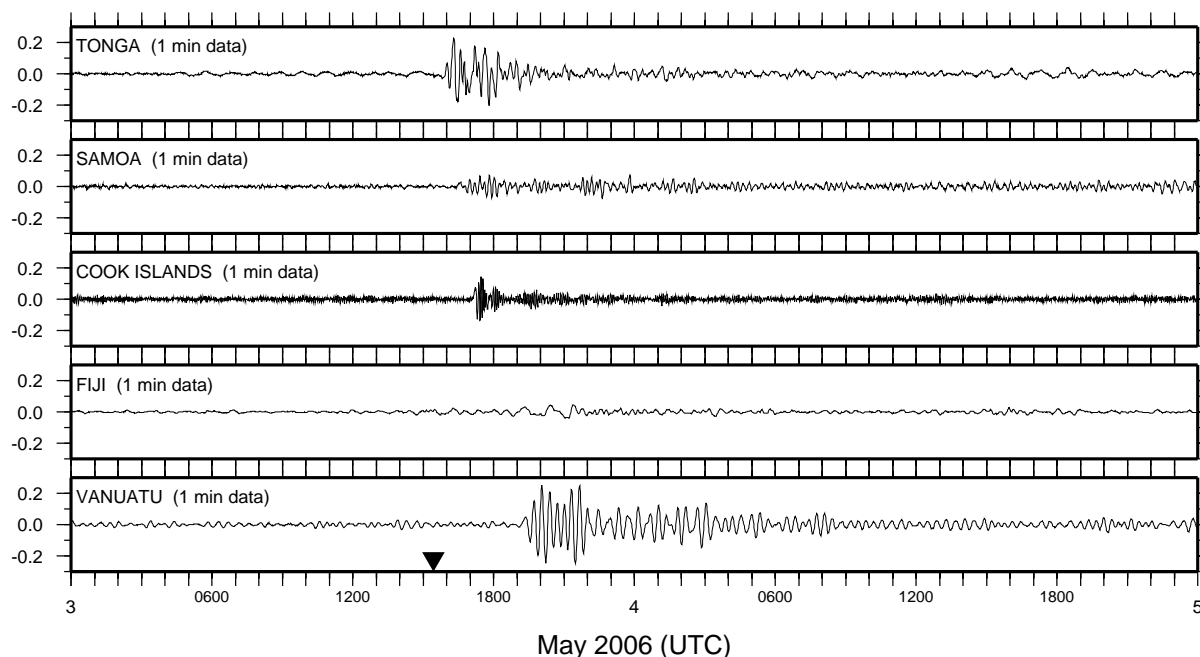
Figure 13. The non-tidal sea level record (m) at SEAFRAME stations following a tsunamigenic earthquake near Tonga at 15:27 UTC on 3 May 2006.
