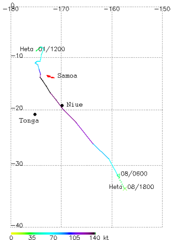
Figure 9. Track of Tropical Cyclone Heta, January 2004
