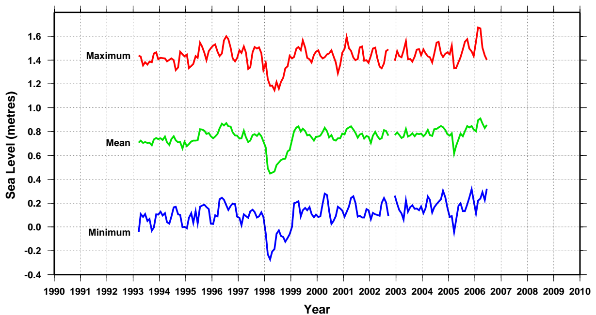
Monthly sea level at Apia SEAFRAME gauge
