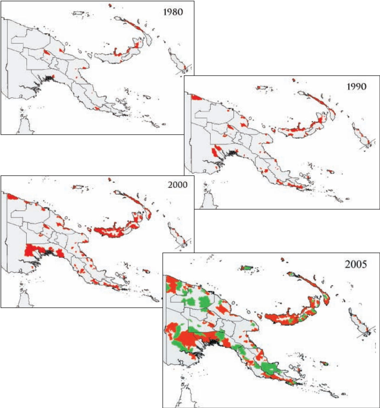
Figure 8: This time series shows the sequential allocation of forest areas to the logging industry between 1980 and 2005. Areas in red are allocated while areas in green are designated as production forests.
