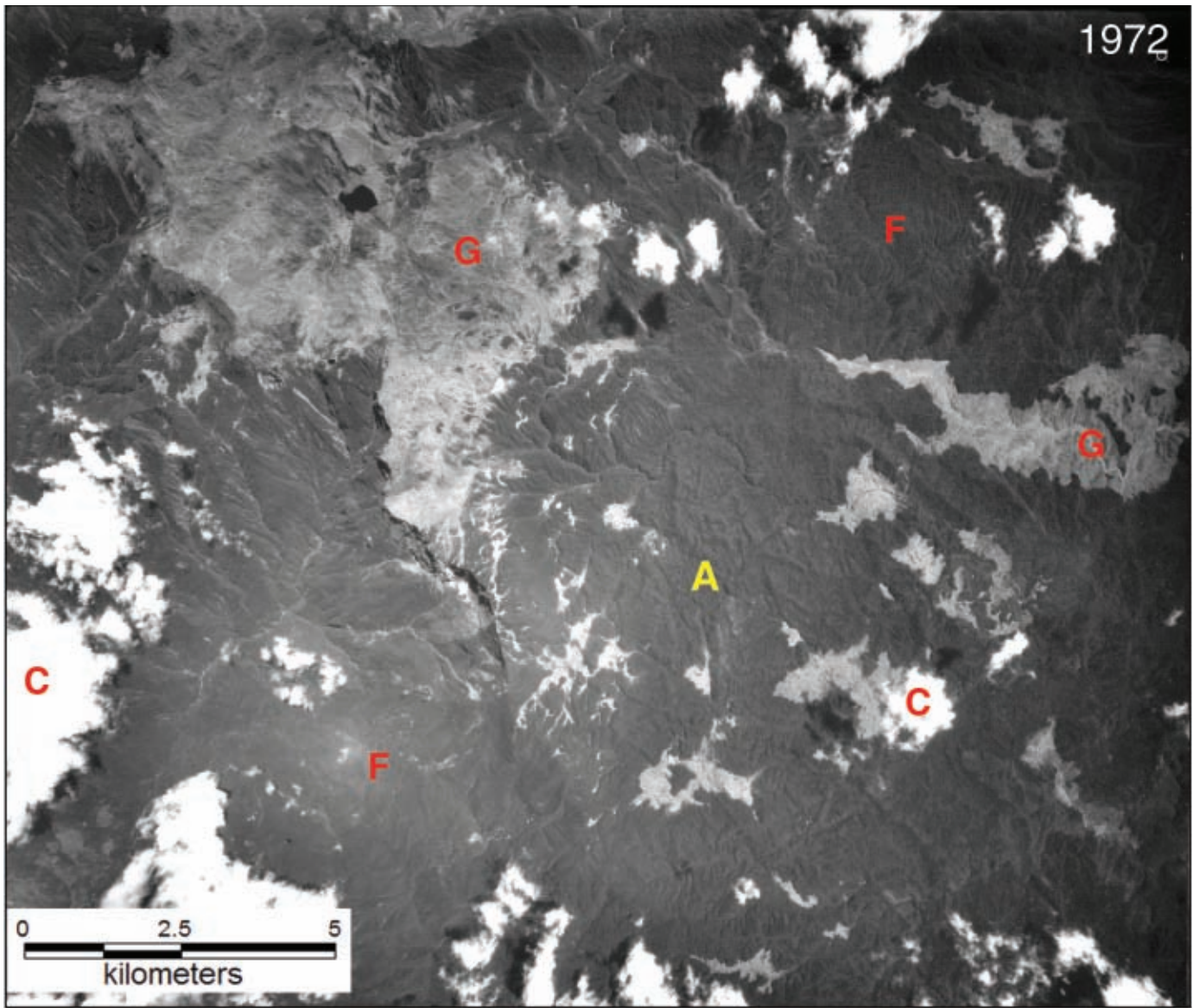
Figure 32: Deforestation on in the Saruwaget Ranges, Huon Peninsula, Morobe Province.
