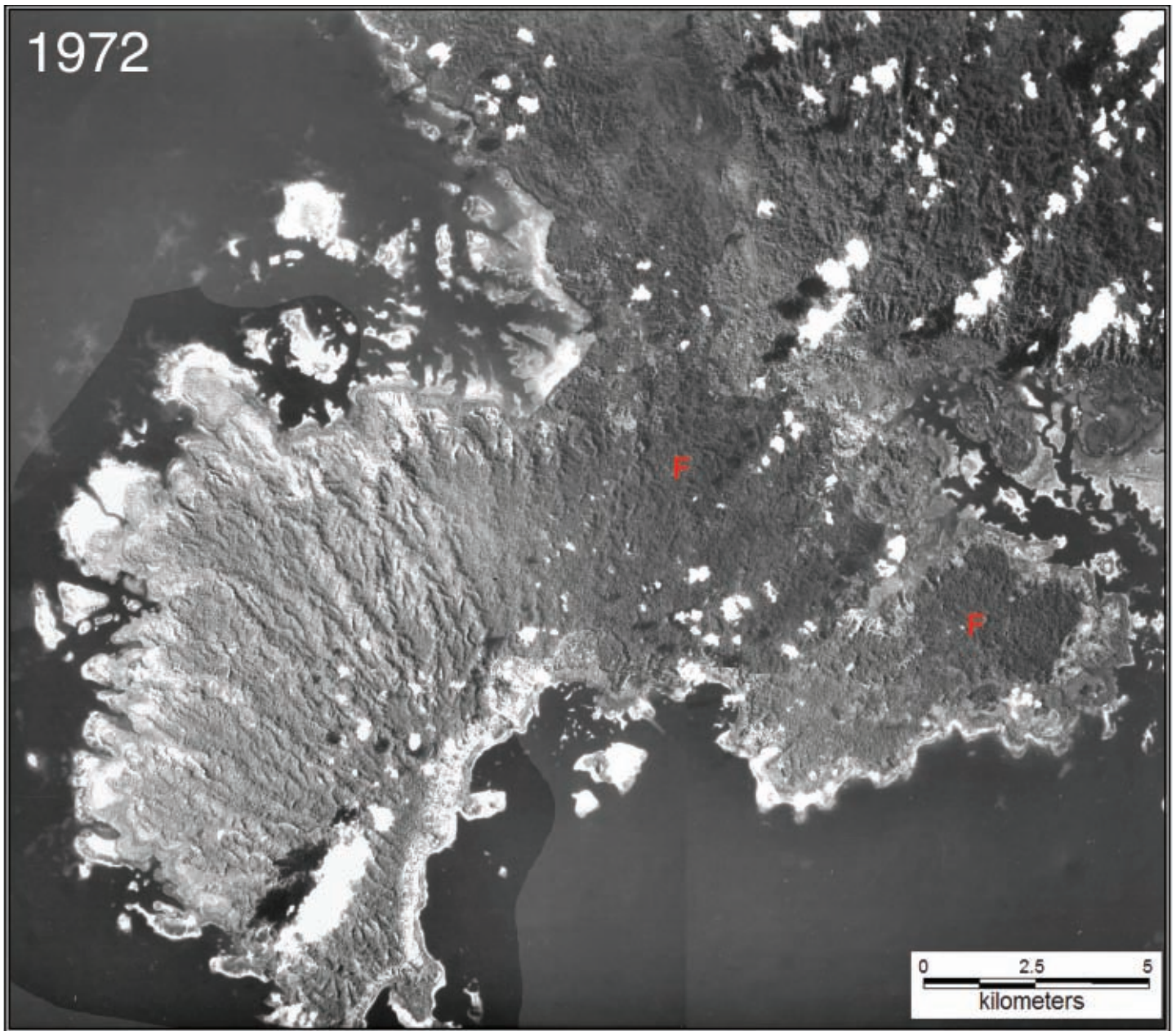
Figure 23: Logging in the south-west of Manus Island.
