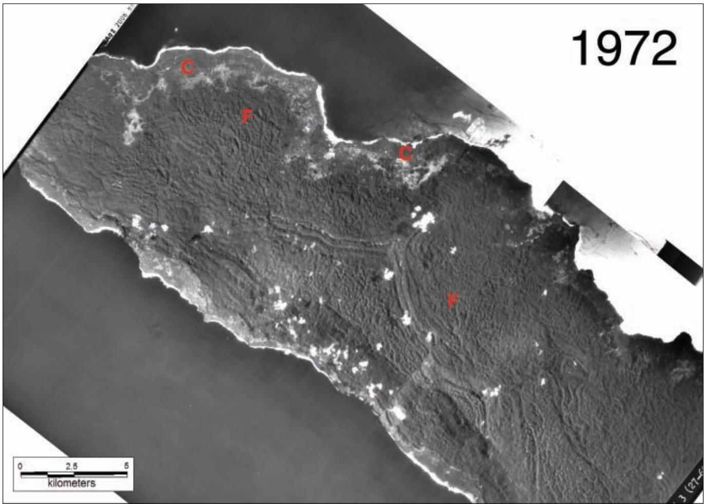
Figure 26: Deforestation in central New Ireland.
