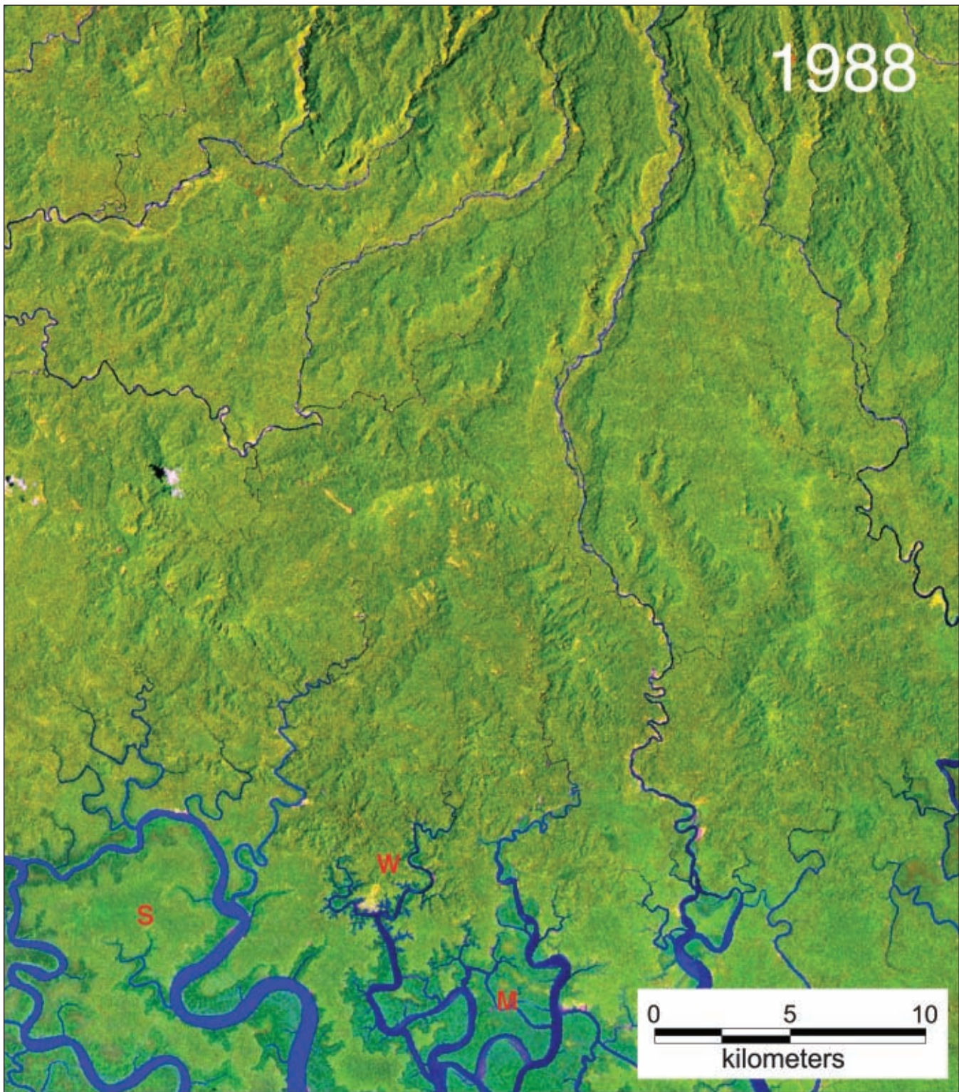
Figure 22: A section of the East Kikori logging operation in Gulf Province. Above, a Landsat TM image from 1988 shows intact primary rainforest across most of the image. Areas of Swamp Forest ( S ) and Mangroves ( M ) are visible in the southern portion of the image. The village of Wowoubo is located with the symbol W . The Landsat ETM+ image on the facing page shows the effects of the logging operation that began around 1995. The roading of the logging operation is clearly visible as are areas of deforestation associated with log ponds and high intensity cutting. The network of tracks and associated damage is typical of lowland logging operations.
