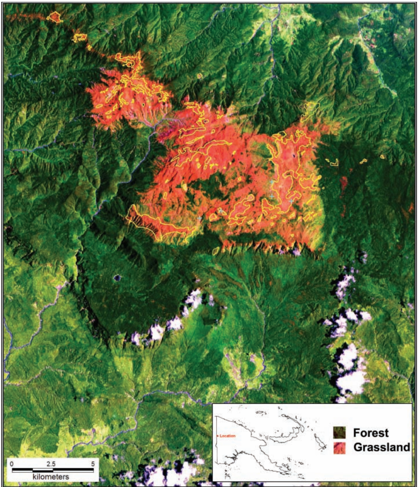
Figure 30: Deforestation on Mt Auriga and Mt Kusiwigasi (Scorpio) (4,015), Star Mountains, Western and West Sepik Provinces.
