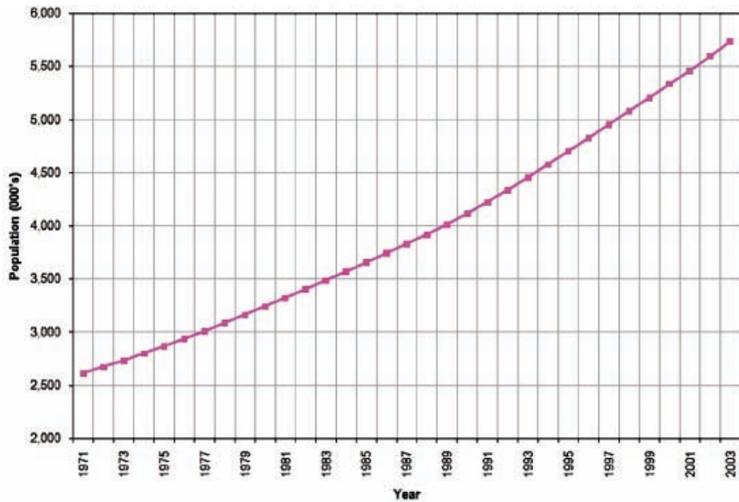
Figure 13: Estimates of PNG population (in thousands) over the period 1961-2003. (FAOSTSAT, 2005).
