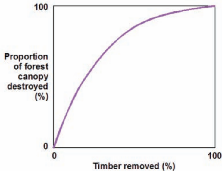
Figure 19: A hypothetical relationship between the area degraded by varying intensities of selective logging.
