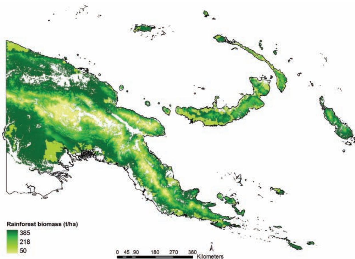
Figure 6: Estimation of biomass across PNG's extant rainforests from all published data gathered in the period 1960-2005.
