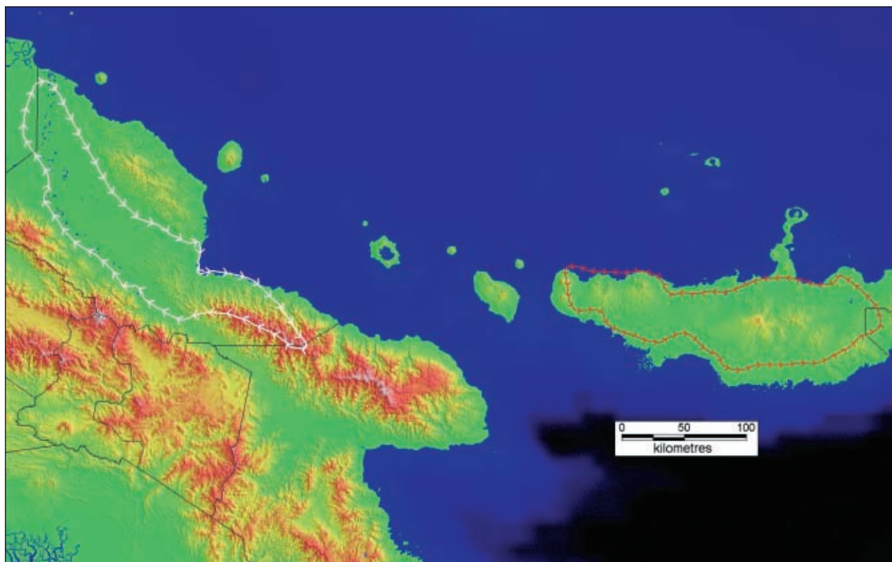
Figure 41: The flight routes used in the aerial surveys of West New Britain (Red) and Madang (White).
