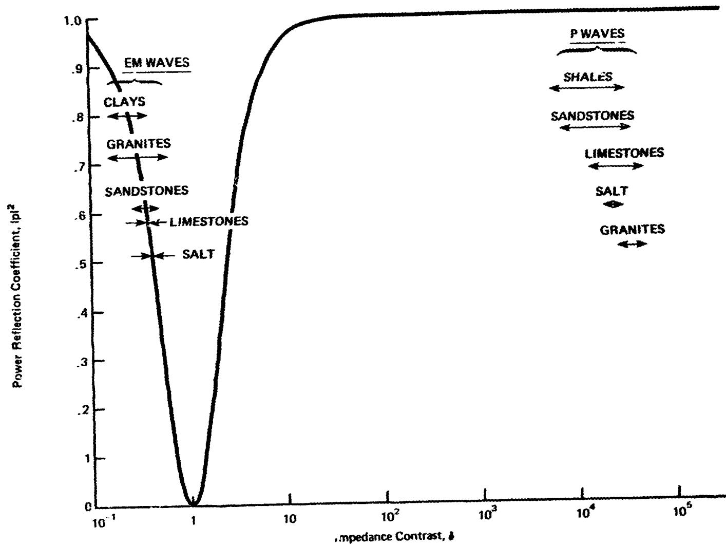
Figure 8 MAXIMUM POWER REFLECTION COEFFICIENT, |\rho|^2 , AS A FUNCTION OF IMPEDANCE CONTRAST, \delta = \eta/\eta_{\text{air}} FOR A SLAB MODEL TUNNEL. THE MAXIMUM OCCURS FOR TUNNEL WIDTHS EQUAL TO \lambda_{\text{air}}/4, 3\lambda_{\text{air}}/4, 5\lambda_{\text{air}}/4 , etc. ALSO SHOWN ON THE FIGURE ARE THE RANGES OF \delta EXPECTED FOR ELECTROMAGNETIC AND COMPRESSIONAL SEISMIC WAVES IN A VARIETY OF GEOLOGICAL MATERIALS - see Table III.
