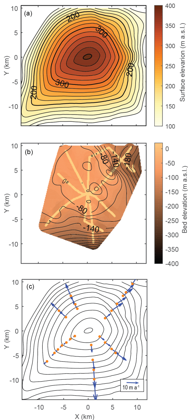
Figure 2. Ice surface (a), bed topography (b) and ice-flow field (c) of the ice rise. The local coordinates are parallel to the polar stereographic coordinates EPSG3031 and centered at the ice-rise summit. (a, b) Elevation contours are 20m intervals. In panel b, radar profiles used to derive the bed topography are highlighted in yellow to show the data availability. Kinematic GPS survey locations are shown in Fig. 1b. (c) Surface ice-flow velocities (blue arrows originated from orange circles) overlaid on surface topography (30-m-interval contours). There are more GPS stakes near the summit (Fig. 1b), which did not give significant results.
