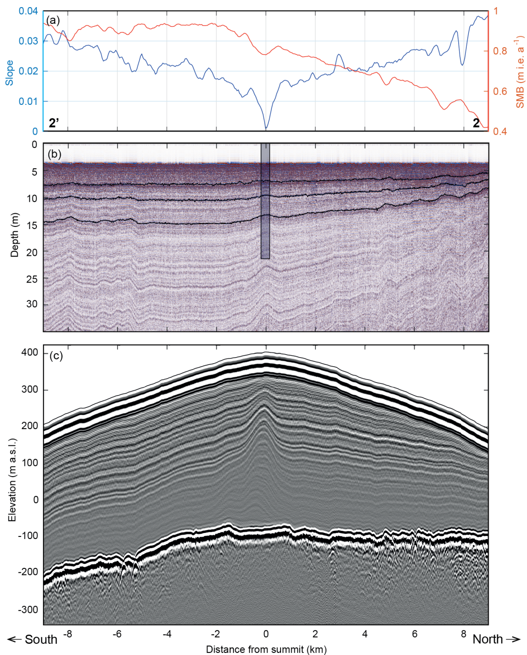
Figure 3. Cross sections of the ice rise along the flowline 2–2' (Fig. 1b). (a) Surface slope (absolute number, left axis) and SMB (right axis). (b) 400-MHz radargram. Three englacial reflectors are highlighted, which are dated with the 23-m-long firn core (vertical bar) and used to determine SMB. (c) 2-MHz radargram. Data are shifted using the GPS-measured surface elevations to show the topography.
