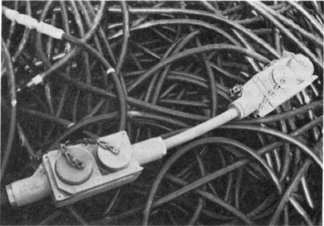
Seismic cable. Note cableheads.
