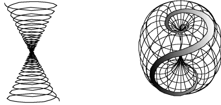
Left, the double vortex creating the torus on the right!
