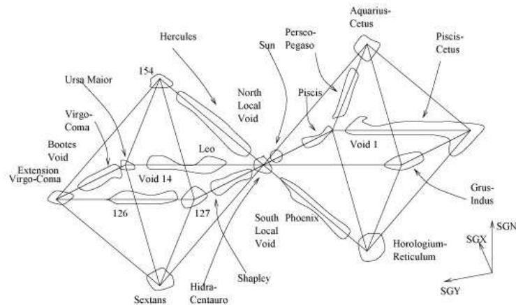
Octahedron clustering of galaxies in the universe
