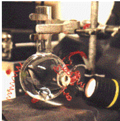
Sonoluminescence experiment
