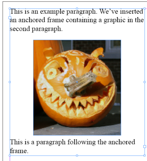
Figure 41. Inline Graphic
