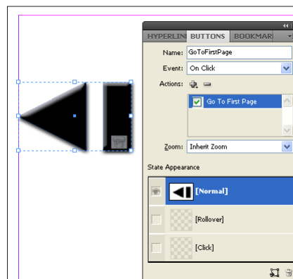
Figure 25. Button
