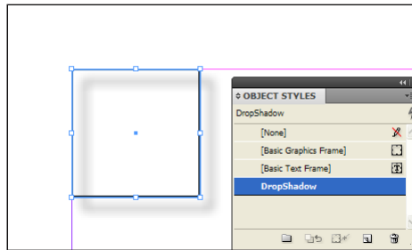
Figure 59. ObjectStyle
