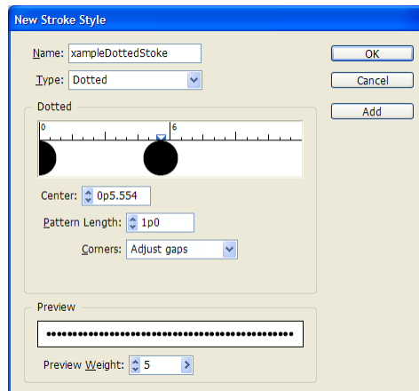
Figure 54. DottedStrokeStyle
