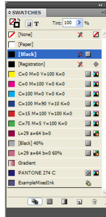
Figure 44. InDesign Swatches
