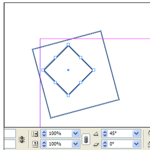
Figure 18. Inner Rectangle
