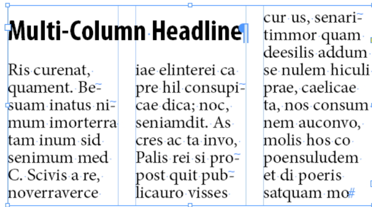
Figure 35. Multi-Column Paragraph
