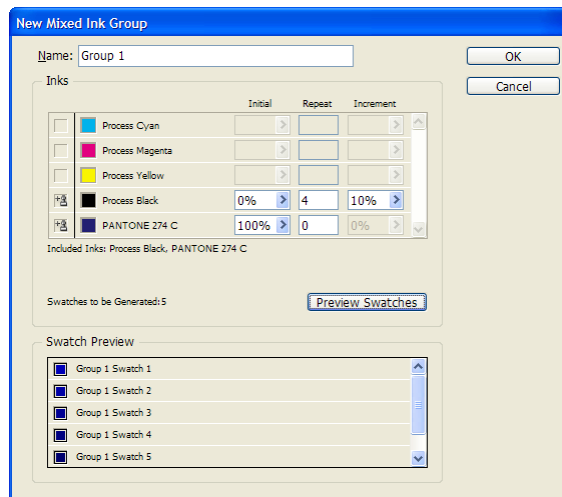
Figure 51. MixedInkGroup
