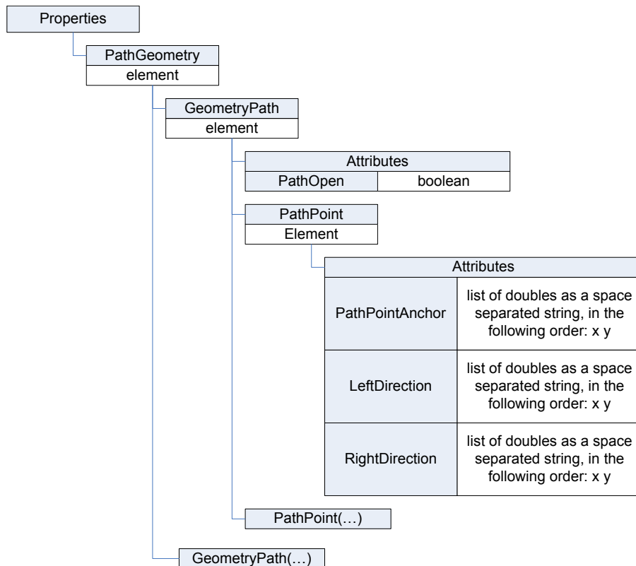
Figure 8. PathGeometry Element
